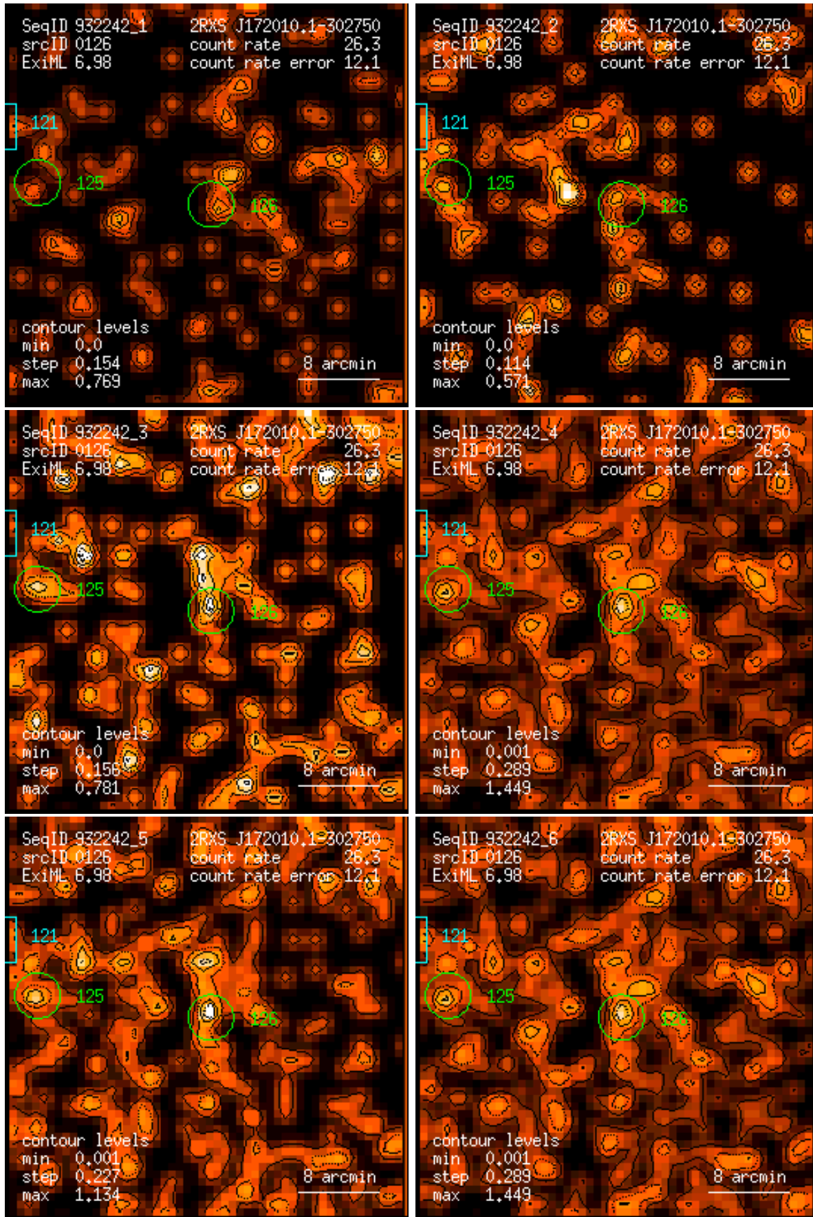
Figure 126: RASS 932242: detection 0126: band rate images, Gaussian filter: (1) PSPC channels 11 – 41, (2) 52 – 90, (3) 91 – 201, (4) 11 – 235, (5) 52 – 201, (6) 11 – 201. Broad band rates in counts/ks. Band rate contour levels in counts/ks/arcmin 2 .
