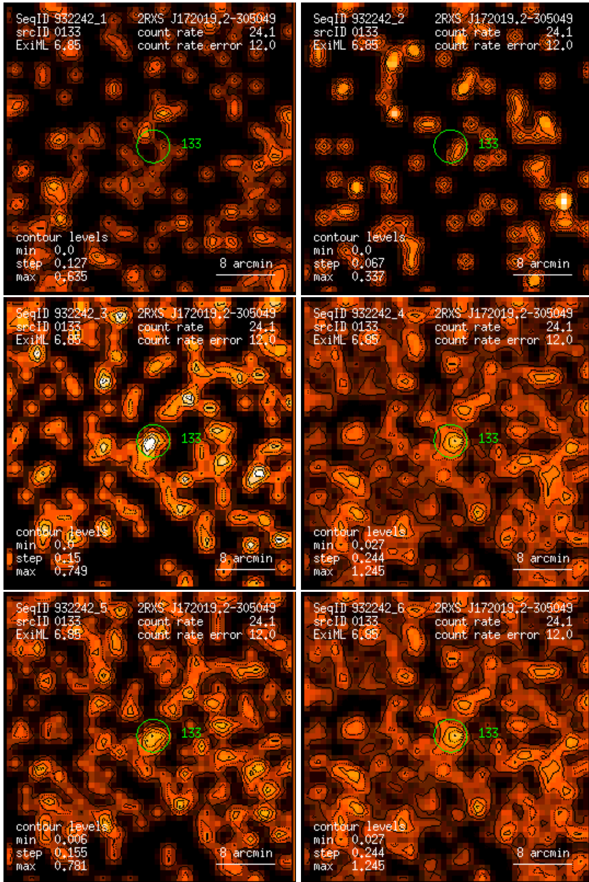
Figure 133: RASS 932242: detection 0133: band rate images, Gaussian filter: (1) PSPC channels 11 – 41, (2) 52 – 90, (3) 91 – 201, (4) 11 – 235, (5) 52 – 201, (6) 11 – 201. Broad band rates in counts/ks. Band rate contour levels in counts/ks/arcmin 2 .
