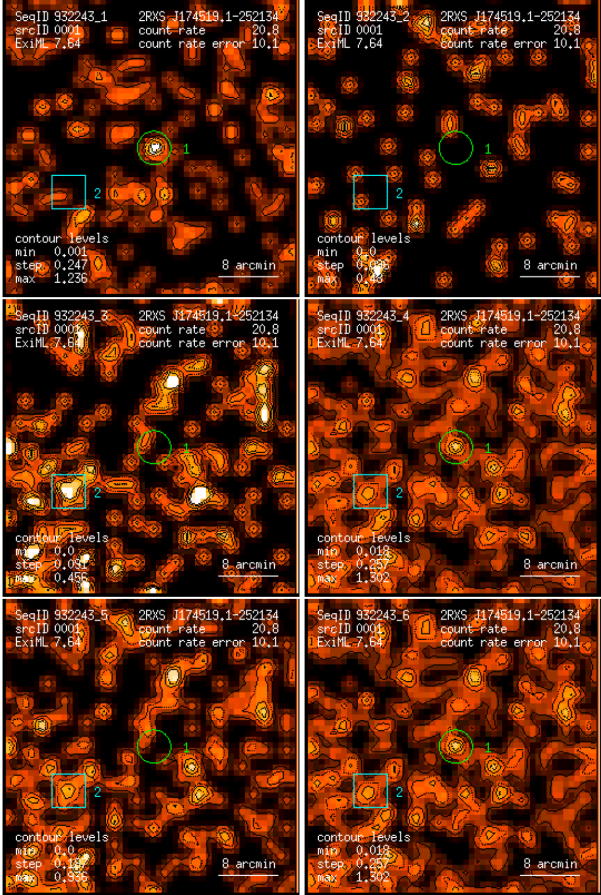
Figure 1: RASS 932243: detection 0001: band rate images, Gaussian filter: (1) PSPC channels 11 – 41, (2) 52 – 90, (3) 91 – 201, (4) 11 – 235, (5) 52 – 201, (6) 11 – 201. Broad band rates in counts/ks. Band rate contour levels in counts/ks/arcmin 2 .
