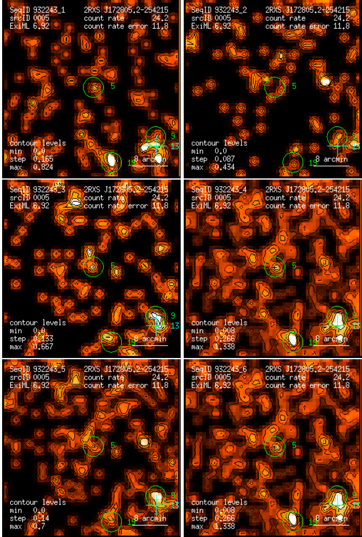
Figure 5: RASS 932243: detection 0005: band rate images, Gaussian filter: (1) PSPC channels 11 – 41, (2) 52 – 90, (3) 91 – 201, (4) 11 – 235, (5) 52 – 201, (6) 11 – 201. Broad band rates in counts/ks. Band rate contour levels in counts/ks/arcmin 2 .
