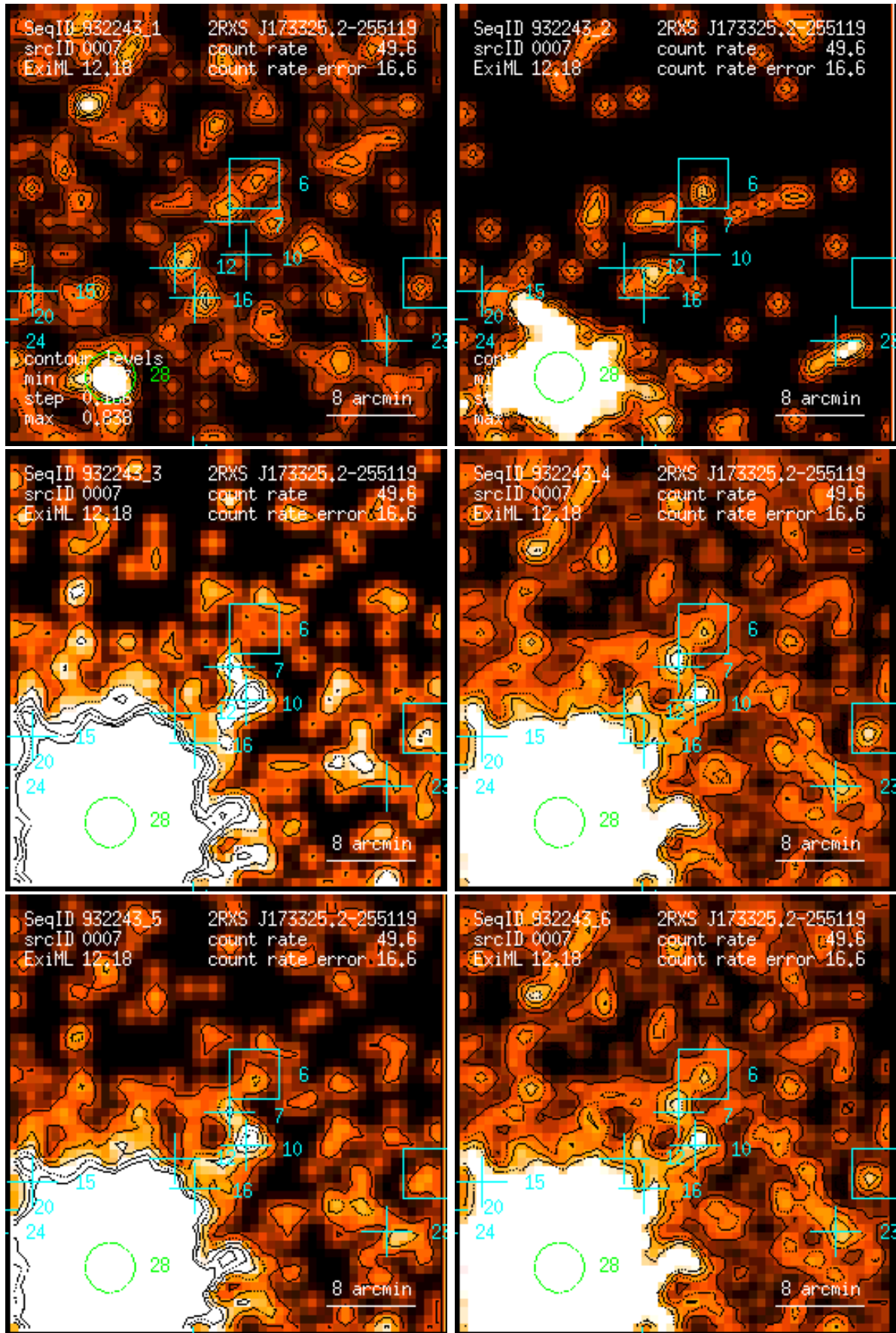
Figure 7: RASS 932243: detection 0007: band rate images, Gaussian filter: (1) PSPC channels 11 – 41, (2) 52 – 90, (3) 91 – 201, (4) 11 – 235, (5) 52 – 201, (6) 11 – 201. Broad band rates in counts/ks. Band rate contour levels in counts/ks/arcmin 2 .
