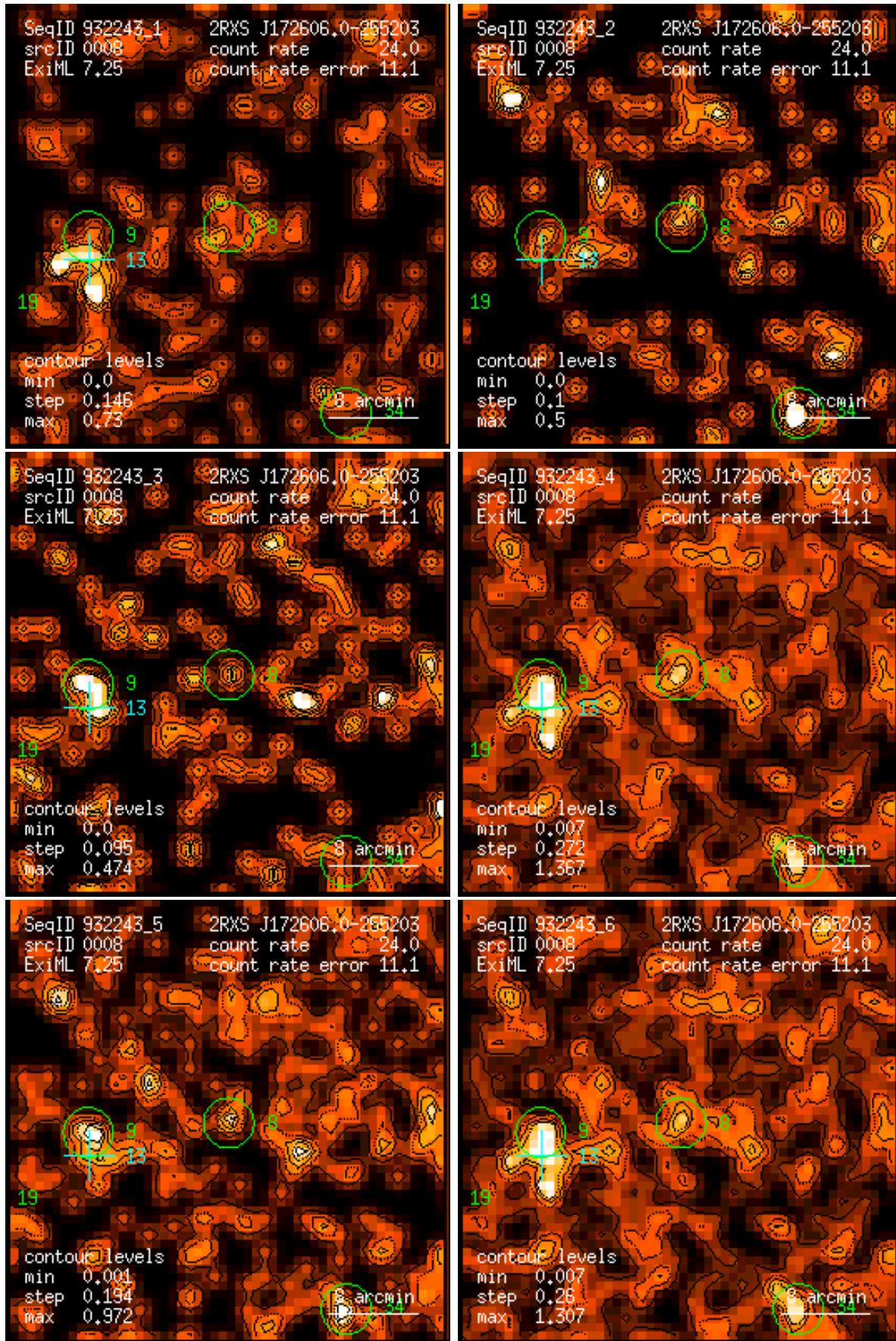
Figure 8: RASS 932243: detection 0008: band rate images, Gaussian filter: (1) PSPC channels 11 – 41, (2) 52 – 90, (3) 91 – 201, (4) 11 – 235, (5) 52 – 201, (6) 11 – 201. Broad band rates in counts/ks. Band rate contour levels in counts/ks/arcmin 2 .
