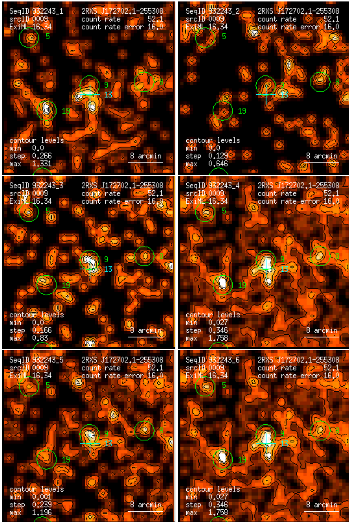
Figure 9: RASS 932243: detection 0009: band rate images, Gaussian filter: (1) PSPC channels 11 – 41, (2) 52 – 90, (3) 91 – 201, (4) 11 – 235, (5) 52 – 201, (6) 11 – 201. Broad band rates in counts/ks. Band rate contour levels in counts/ks/arcmin 2 .
