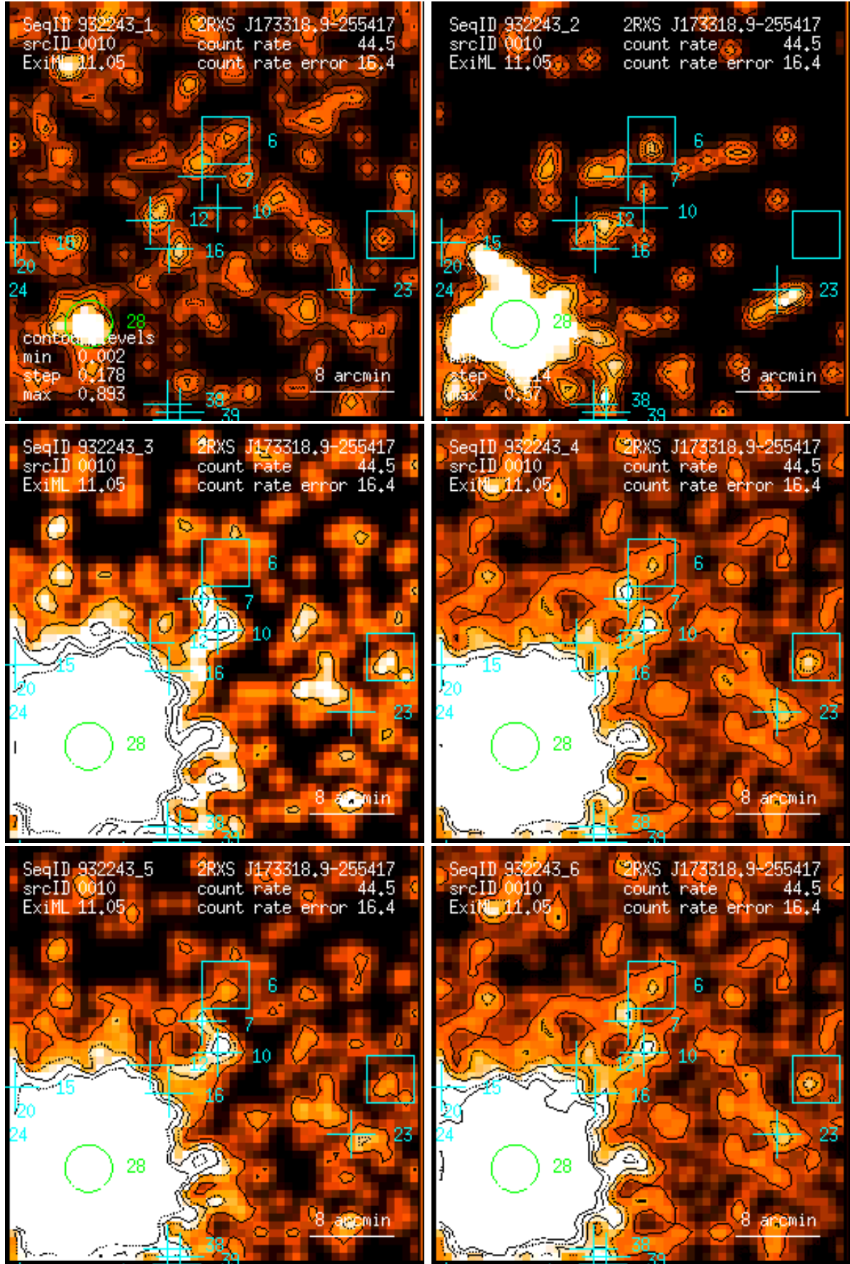
Figure 10: RASS 932243: detection 0010: band rate images, Gaussian filter: (1) PSPC channels 11 – 41, (2) 52 – 90, (3) 91 – 201, (4) 11 – 235, (5) 52 – 201, (6) 11 – 201. Broad band rates in counts/ks. Band rate contour levels in counts/ks/arcmin 2 .
