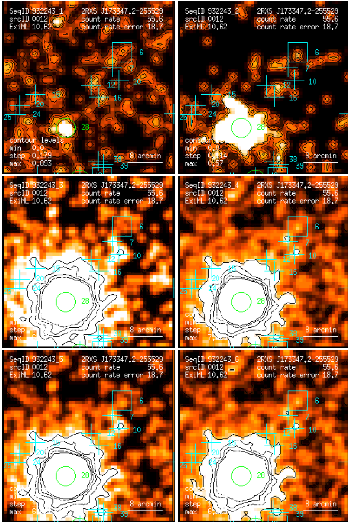
Figure 12: RASS 932243: detection 0012: band rate images, Gaussian filter: (1) PSPC channels 11 – 41, (2) 52 – 90, (3) 91 – 201, (4) 11 – 235, (5) 52 – 201, (6) 11 – 201. Broad band rates in counts/ks. Band rate contour levels in counts/ks/arcmin 2 .
