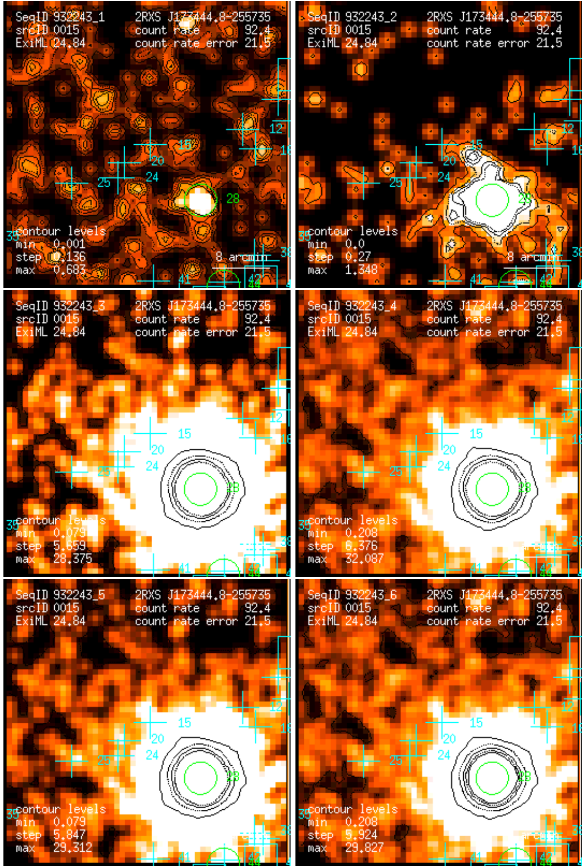
Figure 15: RASS 932243: detection 0015: band rate images, Gaussian filter: (1) PSPC channels 11 – 41, (2) 52 – 90, (3) 91 – 201, (4) 11 – 235, (5) 52 – 201, (6) 11 – 201. Broad band rates in counts/ks. Band rate contour levels in counts/ks/arcmin 2 .
