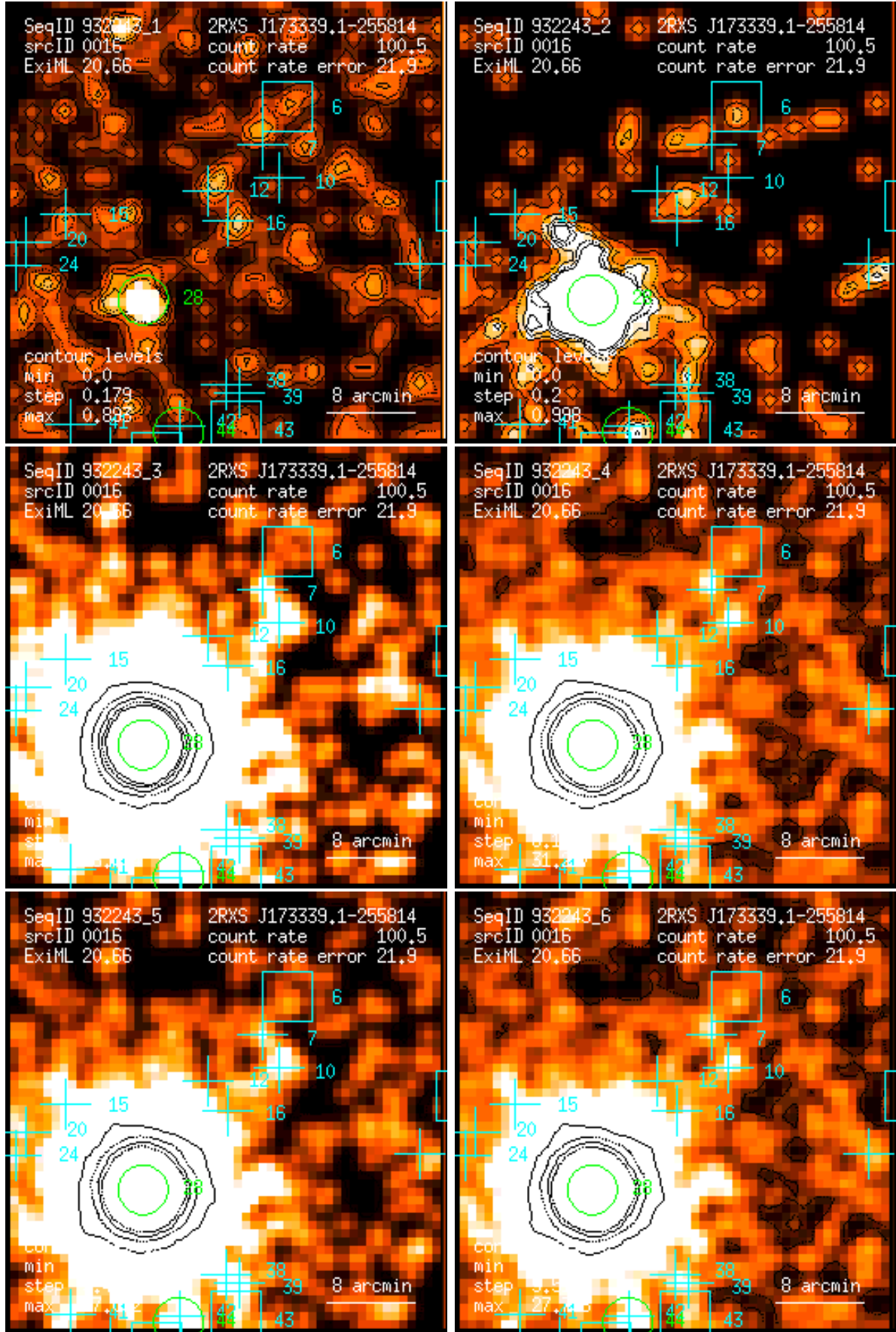
Figure 16: RASS 932243: detection 0016: band rate images, Gaussian filter: (1) PSPC channels 11 – 41, (2) 52 – 90, (3) 91 – 201, (4) 11 – 235, (5) 52 – 201, (6) 11 – 201. Broad band rates in counts/ks. Band rate contour levels in counts/ks/arcmin 2 .
