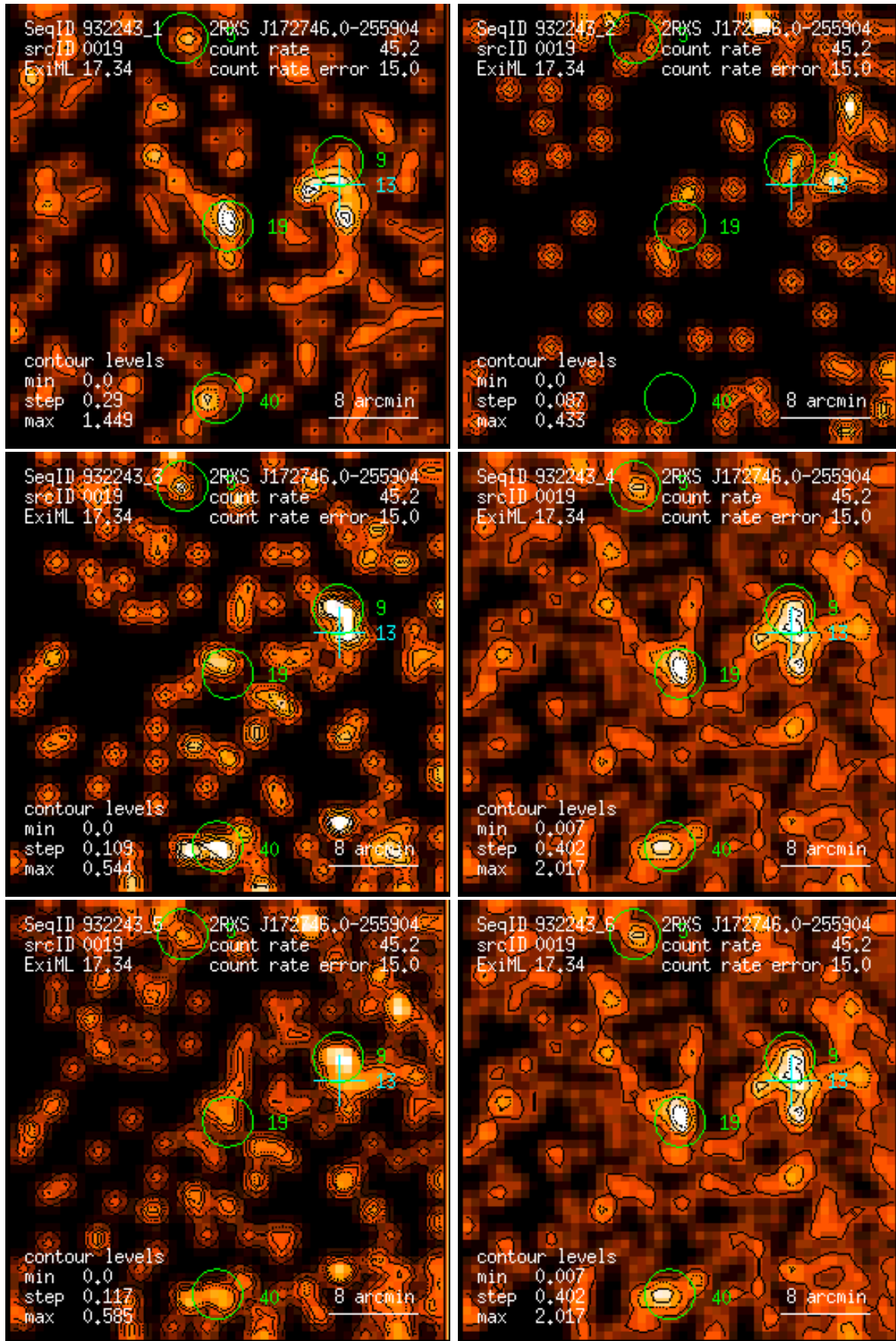
Figure 19: RASS 932243: detection 0019: band rate images, Gaussian filter: (1) PSPC channels 11 – 41, (2) 52 – 90, (3) 91 – 201, (4) 11 – 235, (5) 52 – 201, (6) 11 – 201. Broad band rates in counts/ks. Band rate contour levels in counts/ks/arcmin 2 .
