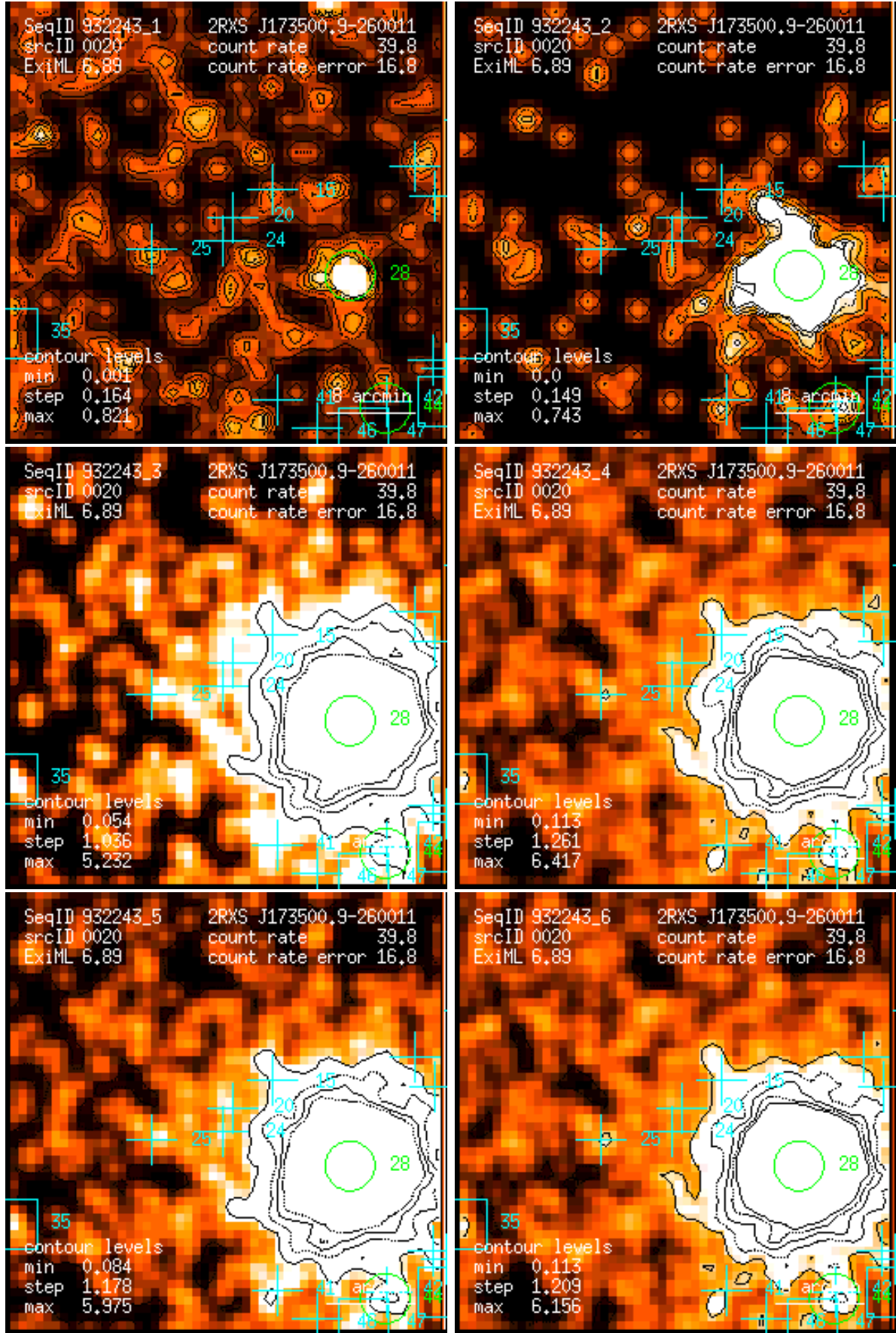
Figure 20: RASS 932243: detection 0020: band rate images, Gaussian filter: (1) PSPC channels 11 – 41, (2) 52 – 90, (3) 91 – 201, (4) 11 – 235, (5) 52 – 201, (6) 11 – 201. Broad band rates in counts/ks. Band rate contour levels in counts/ks/arcmin 2 .
