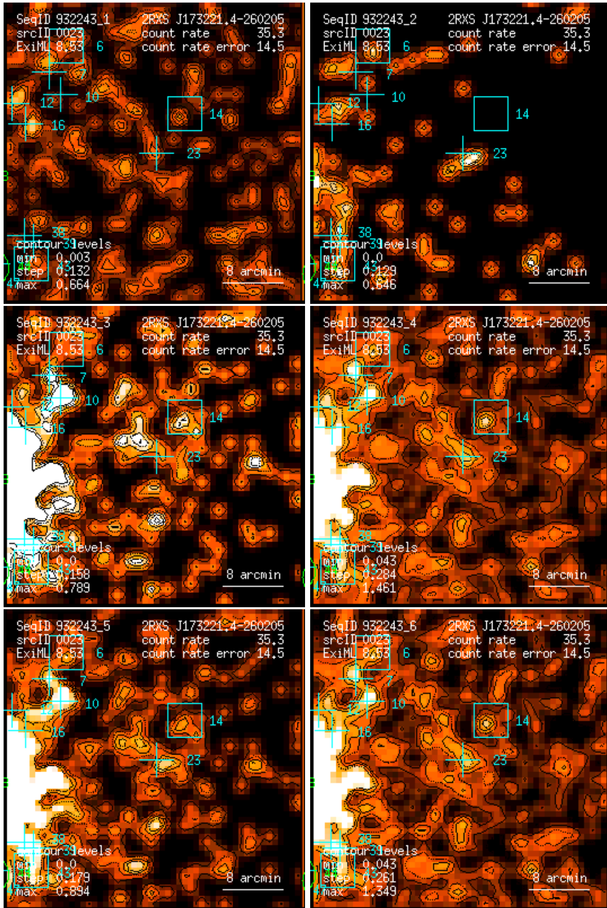
Figure 23: RASS 932243: detection 0023: band rate images, Gaussian filter: (1) PSPC channels 11 – 41, (2) 52 – 90, (3) 91 – 201, (4) 11 – 235, (5) 52 – 201, (6) 11 – 201. Broad band rates in counts/ks. Band rate contour levels in counts/ks/arcmin 2 .
