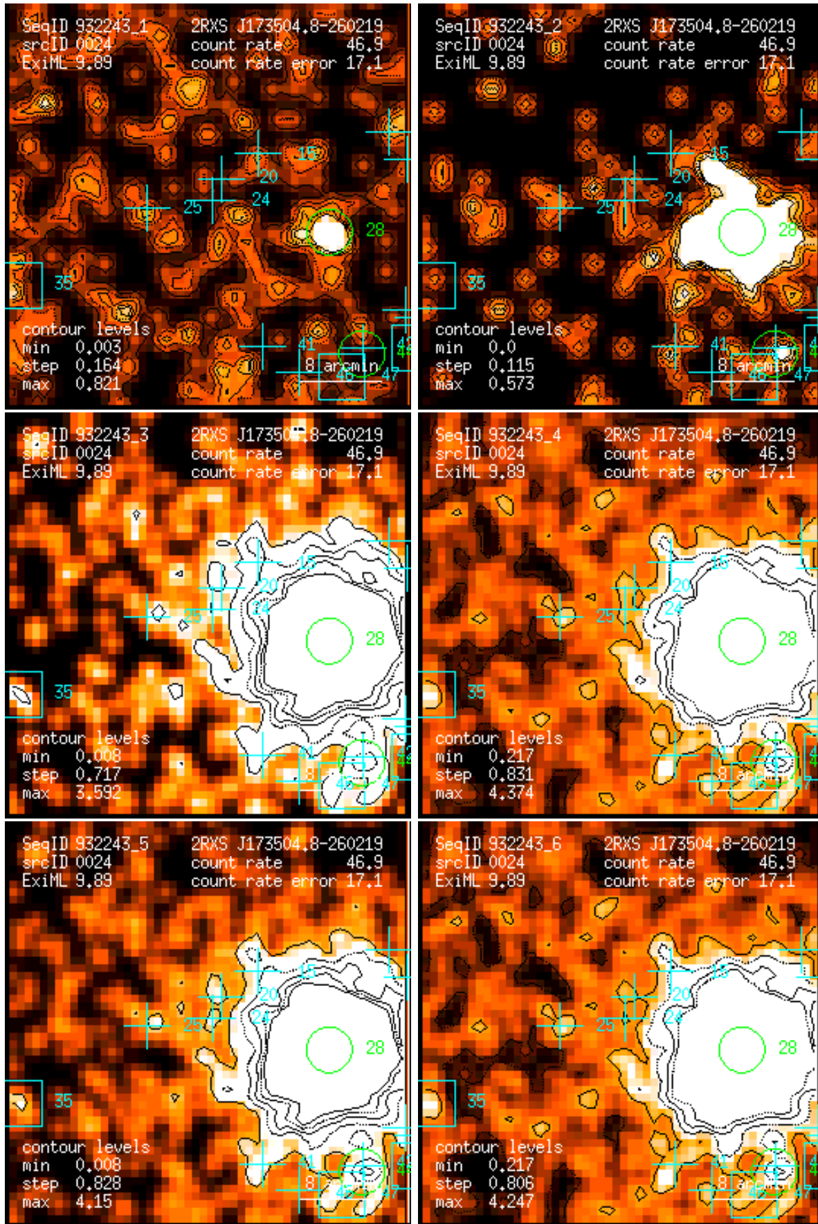
Figure 24: RASS 932243: detection 0024: band rate images, Gaussian filter: (1) PSPC channels 11 – 41, (2) 52 – 90, (3) 91 – 201, (4) 11 – 235, (5) 52 – 201, (6) 11 – 201. Broad band rates in counts/ks. Band rate contour levels in counts/ks/arcmin 2 .
