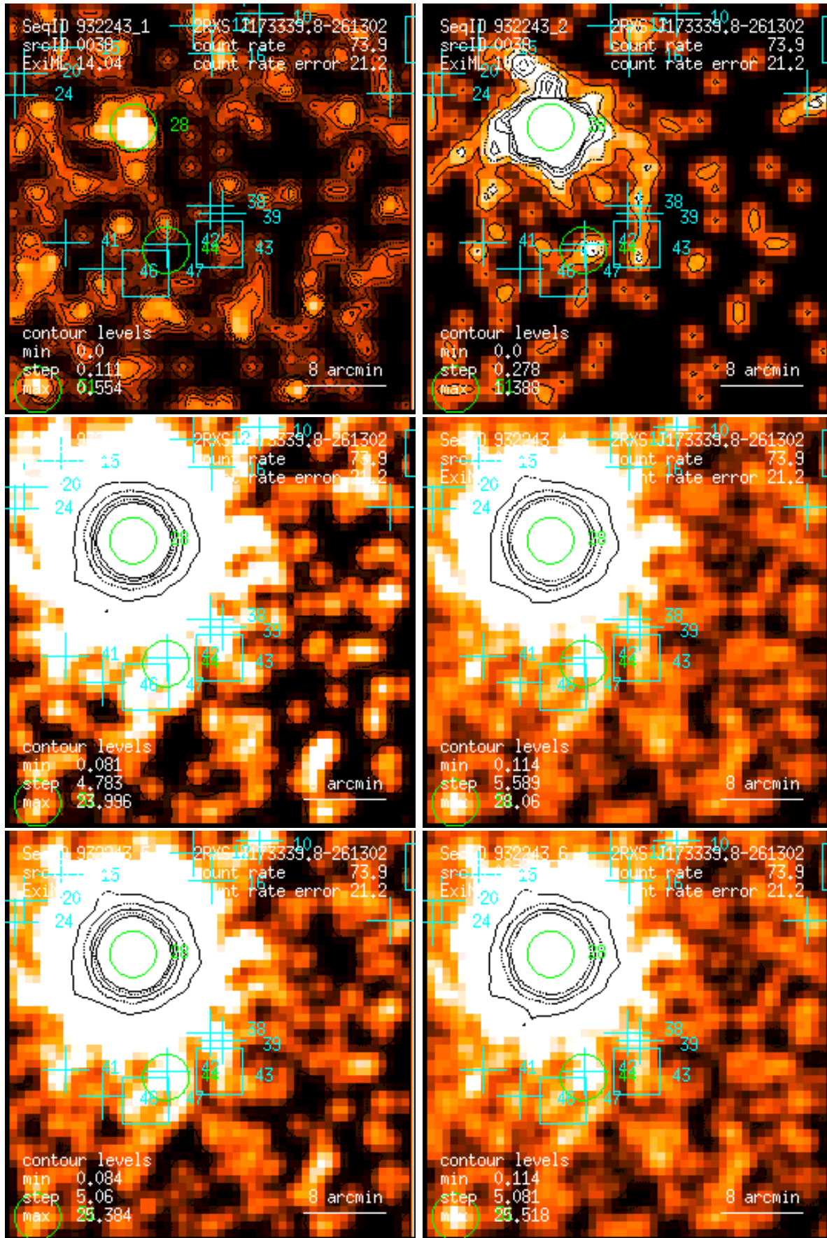
Figure 38: RASS 932243: detection 0038: band rate images, Gaussian filter: (1) PSPC channels 11 – 41, (2) 52 – 90, (3) 91 – 201, (4) 11 – 235, (5) 52 – 201, (6) 11 – 201. Broad band rates in counts/ks. Band rate contour levels in counts/ks/arcmin 2 .
