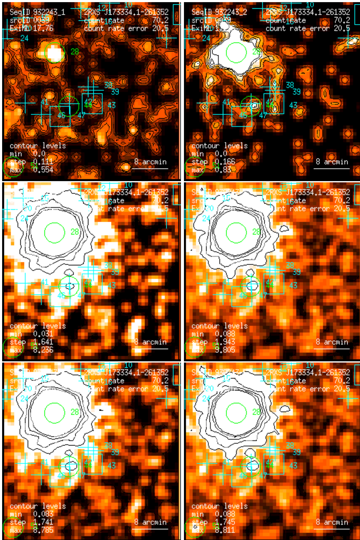
Figure 39: RASS 932243: detection 0039: band rate images, Gaussian filter: (1) PSPC channels 11 – 41, (2) 52 – 90, (3) 91 – 201, (4) 11 – 235, (5) 52 – 201, (6) 11 – 201. Broad band rates in counts/ks. Band rate contour levels in counts/ks/arcmin 2 .
