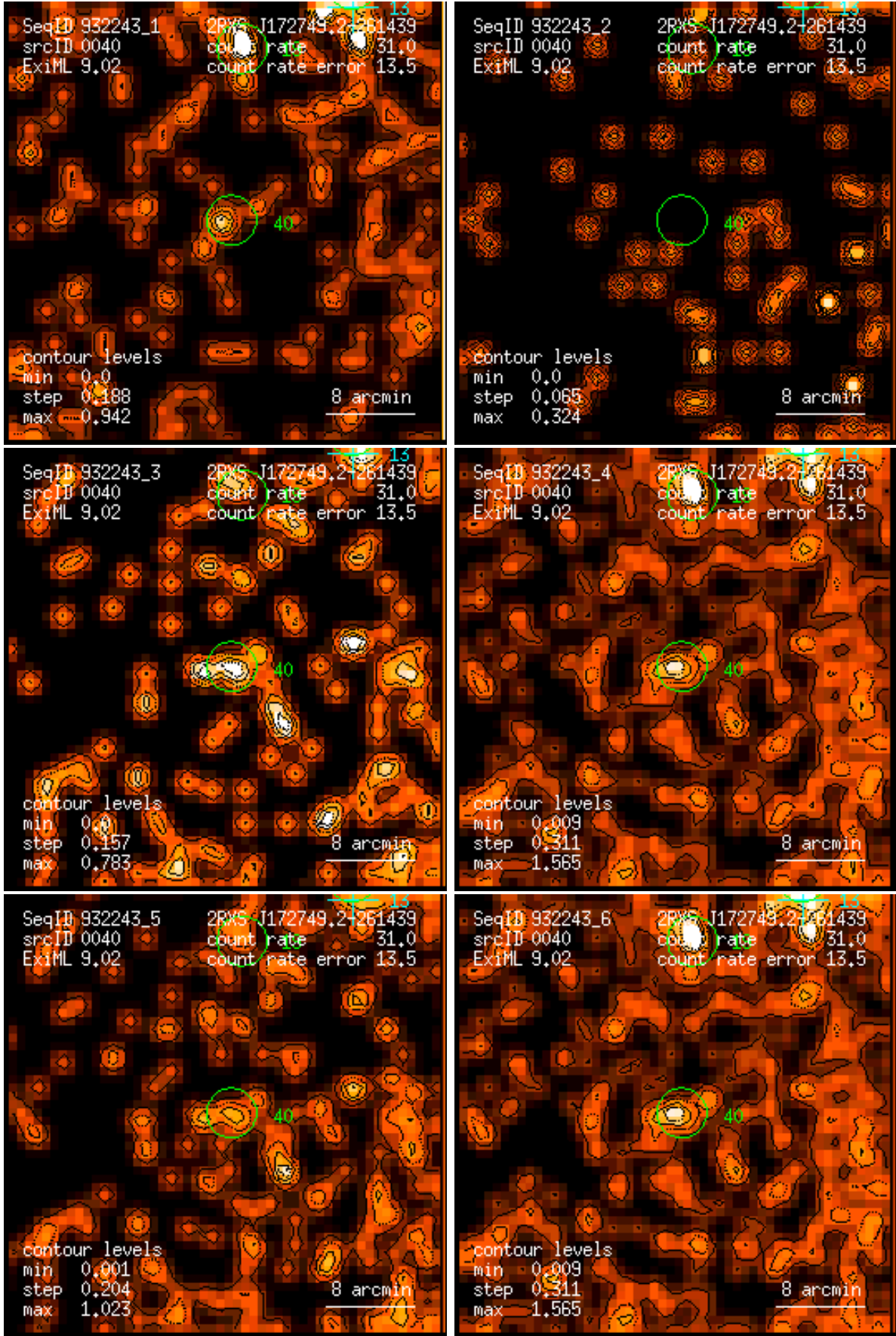
Figure 40: RASS 932243: detection 0040: band rate images, Gaussian filter: (1) PSPC channels 11 – 41, (2) 52 – 90, (3) 91 – 201, (4) 11 – 235, (5) 52 – 201, (6) 11 – 201. Broad band rates in counts/ks. Band rate contour levels in counts/ks/arcmin 2 .
