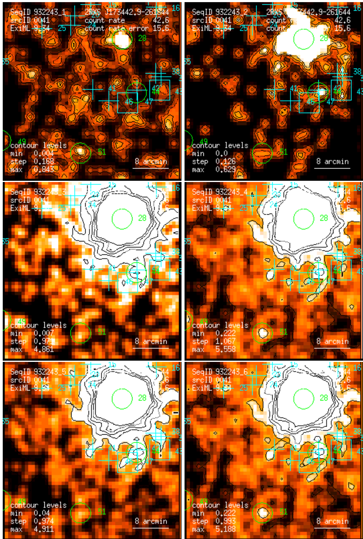
Figure 41: RASS 932243: detection 0041: band rate images, Gaussian filter: (1) PSPC channels 11 – 41, (2) 52 – 90, (3) 91 – 201, (4) 11 – 235, (5) 52 – 201, (6) 11 – 201. Broad band rates in counts/ks. Band rate contour levels in counts/ks/arcmin 2 .
