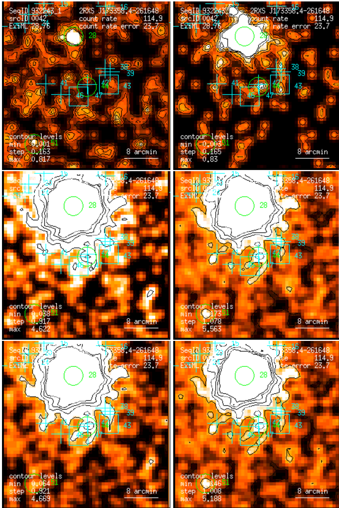
Figure 42: RASS 932243: detection 0042: band rate images, Gaussian filter: (1) PSPC channels 11 – 41, (2) 52 – 90, (3) 91 – 201, (4) 11 – 235, (5) 52 – 201, (6) 11 – 201. Broad band rates in counts/ks. Band rate contour levels in counts/ks/arcmin 2 .
