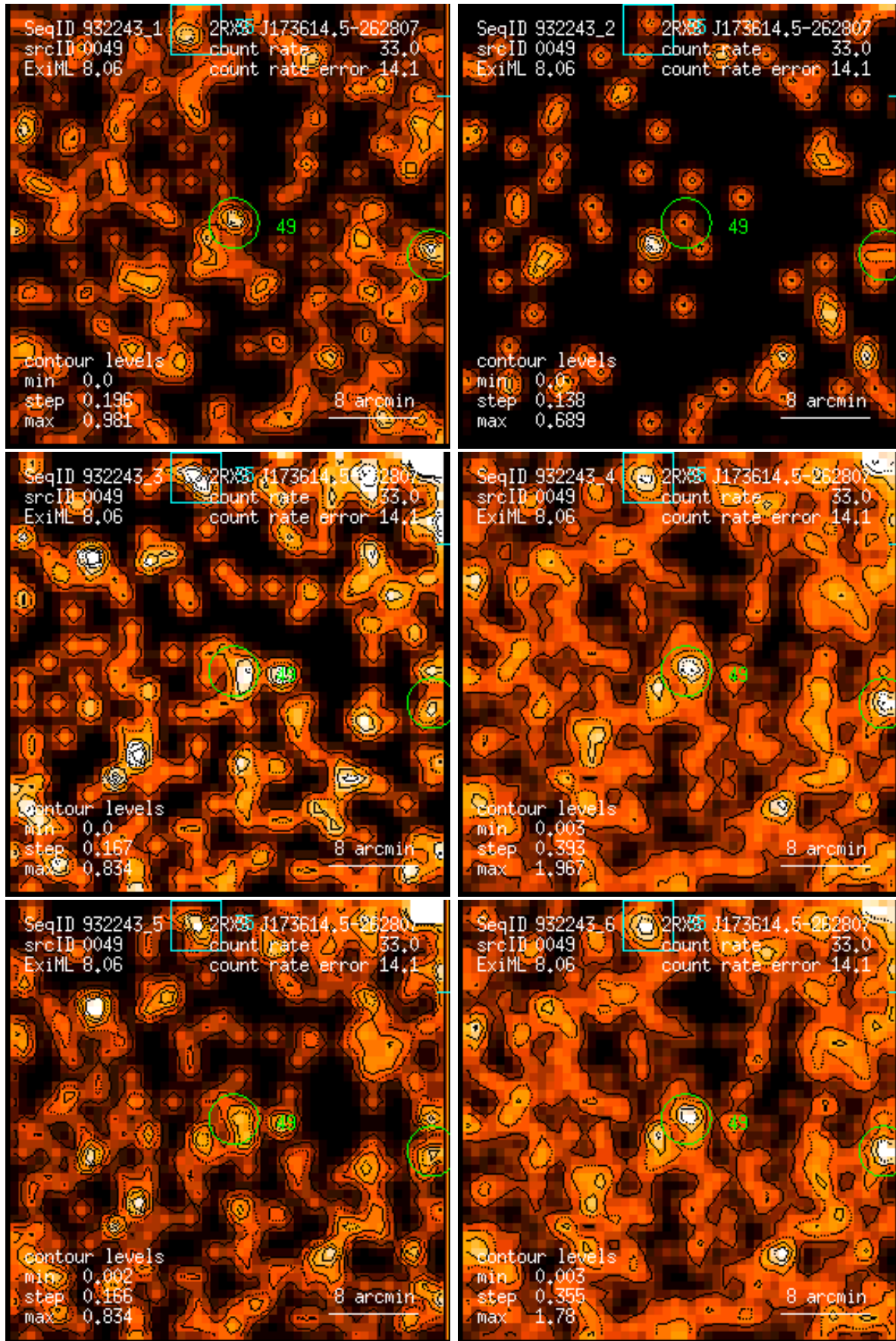
Figure 49: RASS 932243: detection 0049: band rate images, Gaussian filter: (1) PSPC channels 11 – 41, (2) 52 – 90, (3) 91 – 201, (4) 11 – 235, (5) 52 – 201, (6) 11 – 201. Broad band rates in counts/ks. Band rate contour levels in counts/ks/arcmin 2 .
