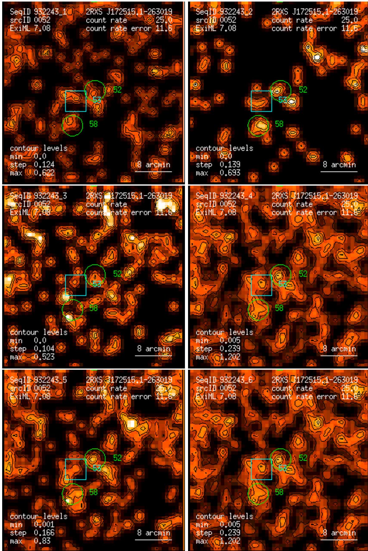
Figure 52: RASS 932243: detection 0052: band rate images, Gaussian filter: (1) PSPC channels 11 – 41, (2) 52 – 90, (3) 91 – 201, (4) 11 – 235, (5) 52 – 201, (6) 11 – 201. Broad band rates in counts/ks. Band rate contour levels in counts/ks/arcmin 2 .
