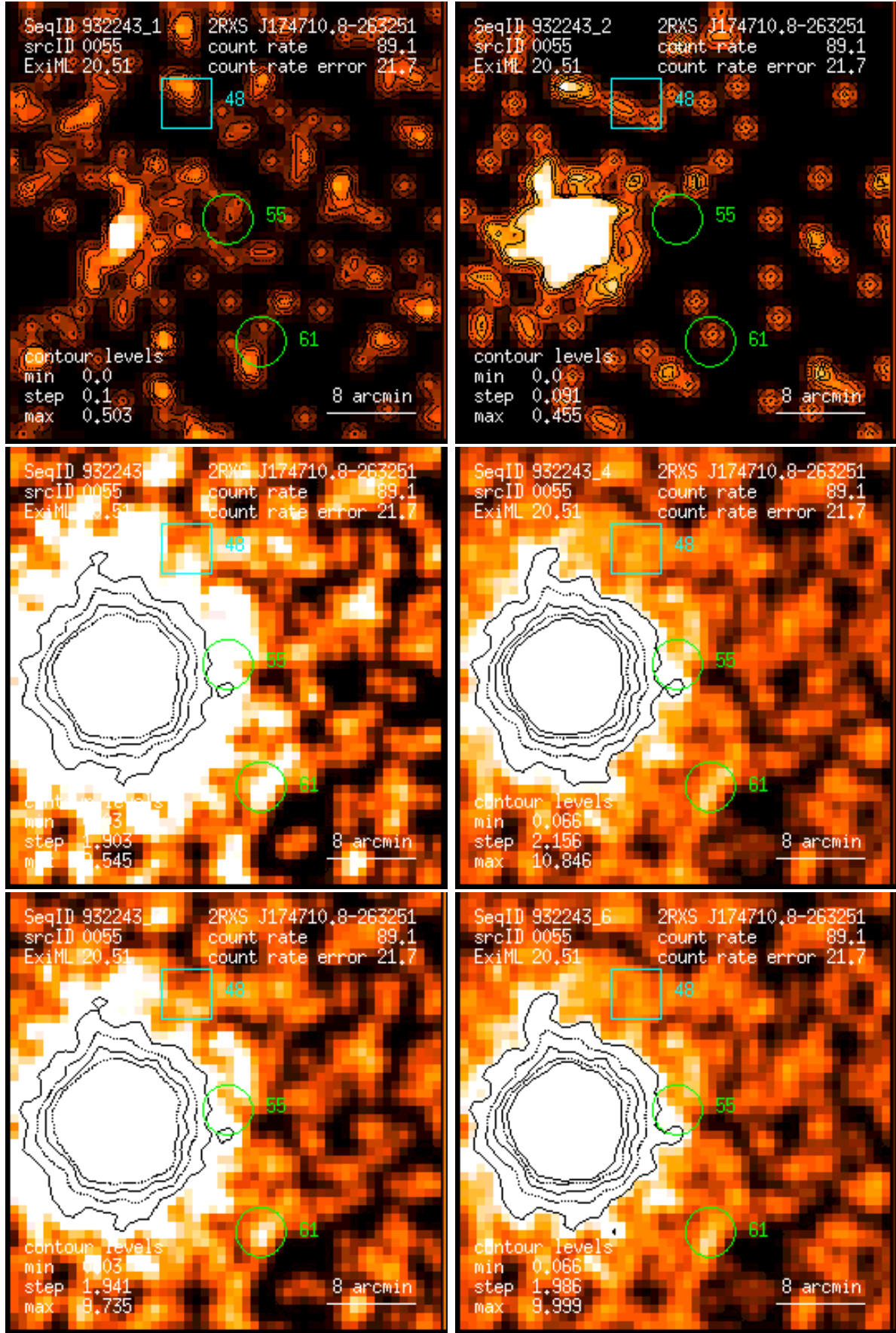
Figure 55: RASS 932243: detection 0055: band rate images, Gaussian filter: (1) PSPC channels 11 – 41, (2) 52 – 90, (3) 91 – 201, (4) 11 – 235, (5) 52 – 201, (6) 11 – 201. Broad band rates in counts/ks. Band rate contour levels in counts/ks/arcmin 2 .
