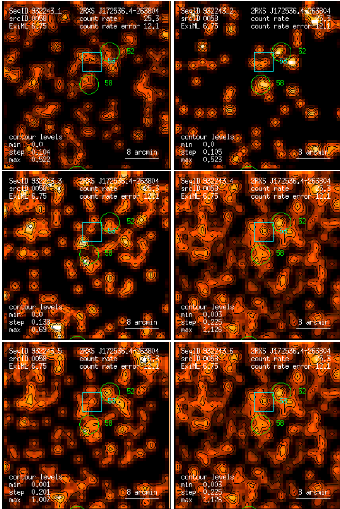
Figure 58: RASS 932243: detection 0058: band rate images, Gaussian filter: (1) PSPC channels 11 – 41, (2) 52 – 90, (3) 91 – 201, (4) 11 – 235, (5) 52 – 201, (6) 11 – 201. Broad band rates in counts/ks. Band rate contour levels in counts/ks/arcmin 2 .
