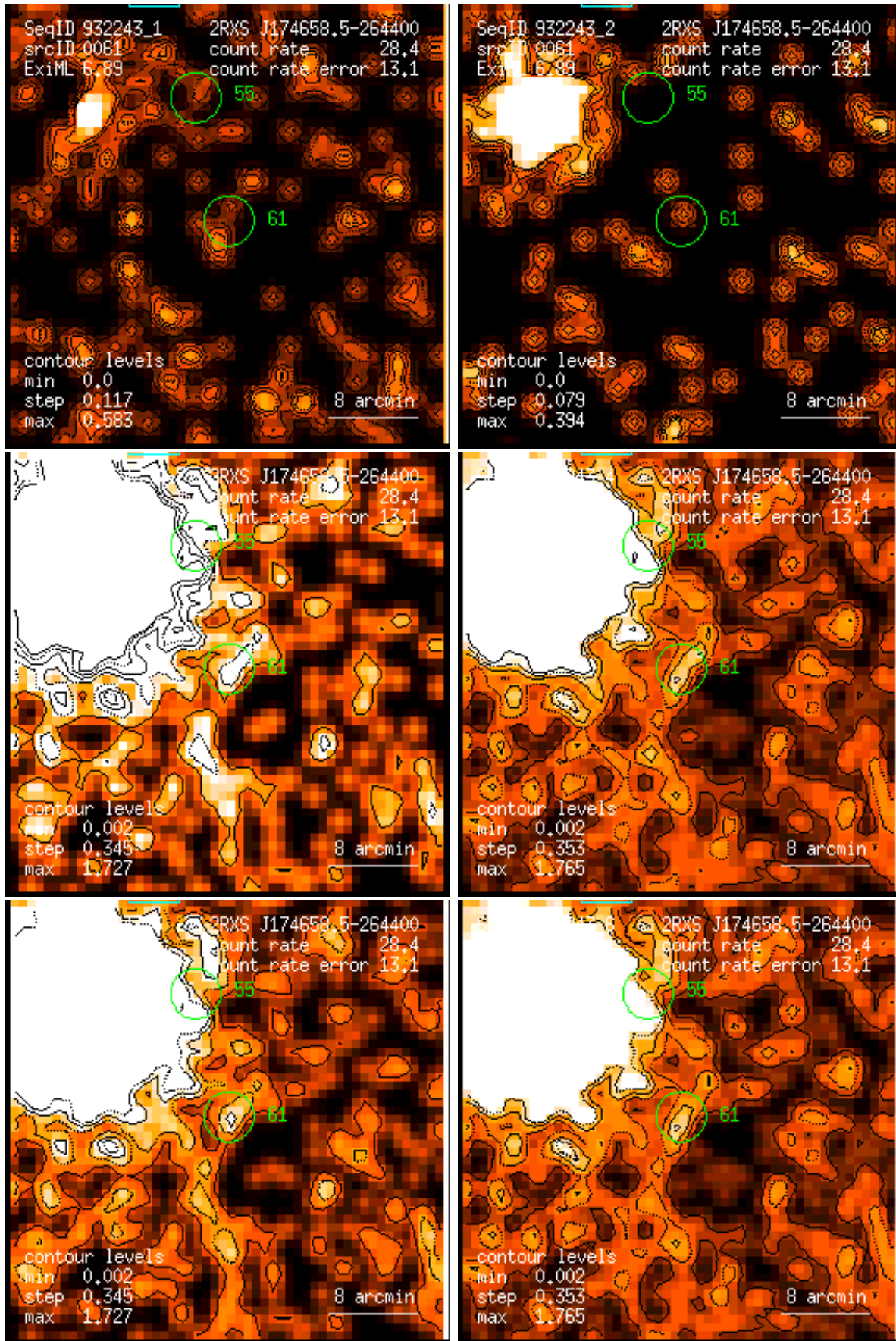
Figure 61: RASS 932243: detection 0061: band rate images, Gaussian filter: (1) PSPC channels 11 – 41, (2) 52 – 90, (3) 91 – 201, (4) 11 – 235, (5) 52 – 201, (6) 11 – 201. Broad band rates in counts/ks. Band rate contour levels in counts/ks/arcmin 2 .
