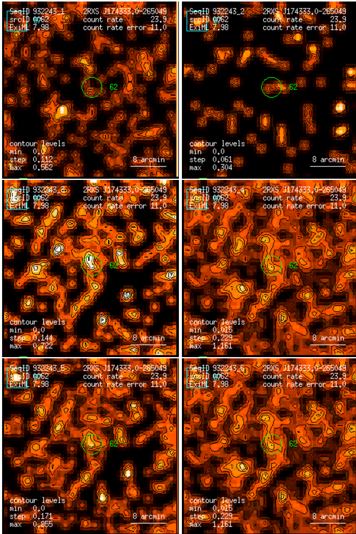
Figure 62: RASS 932243: detection 0062: band rate images, Gaussian filter: (1) PSPC channels 11 – 41, (2) 52 – 90, (3) 91 – 201, (4) 11 – 235, (5) 52 – 201, (6) 11 – 201. Broad band rates in counts/ks. Band rate contour levels in counts/ks/arcmin 2 .
