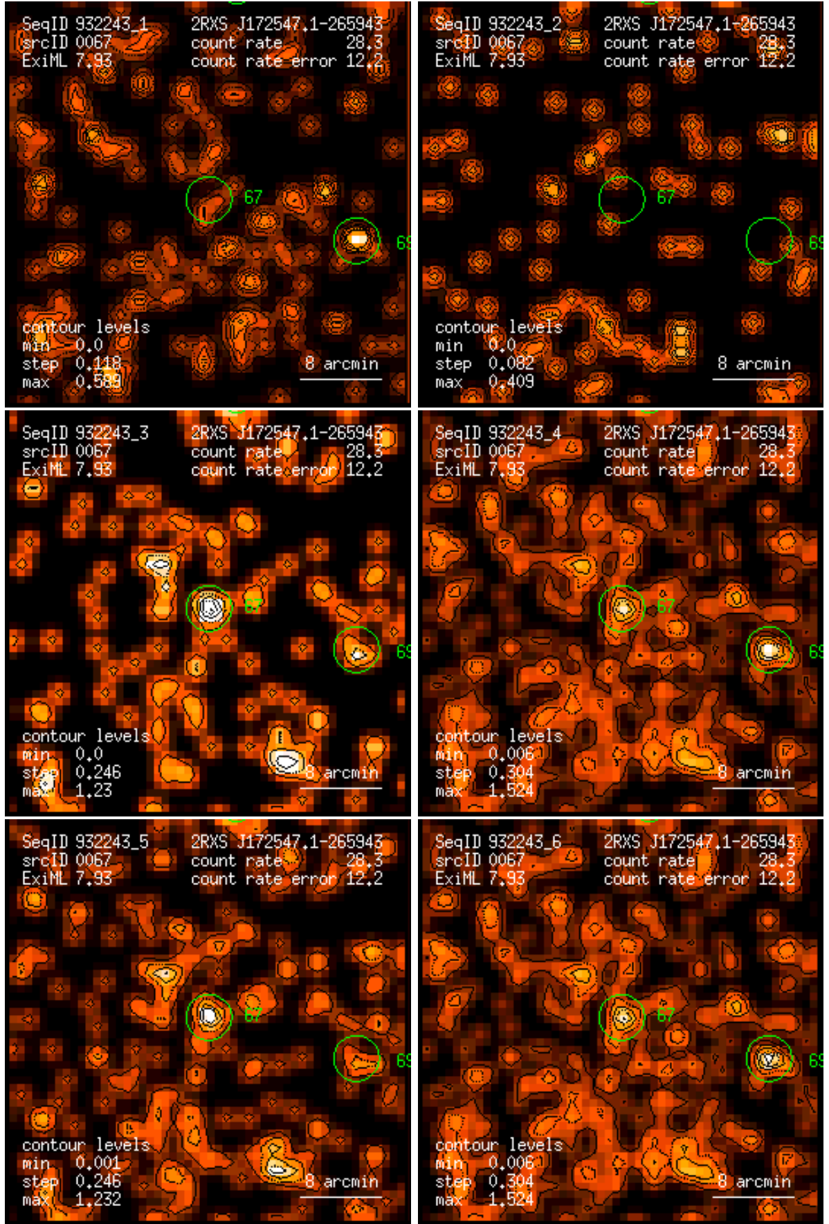
Figure 67: RASS 932243: detection 0067: band rate images, Gaussian filter: (1) PSPC channels 11 – 41, (2) 52 – 90, (3) 91 – 201, (4) 11 – 235, (5) 52 – 201, (6) 11 – 201. Broad band rates in counts/ks. Band rate contour levels in counts/ks/arcmin 2 .
