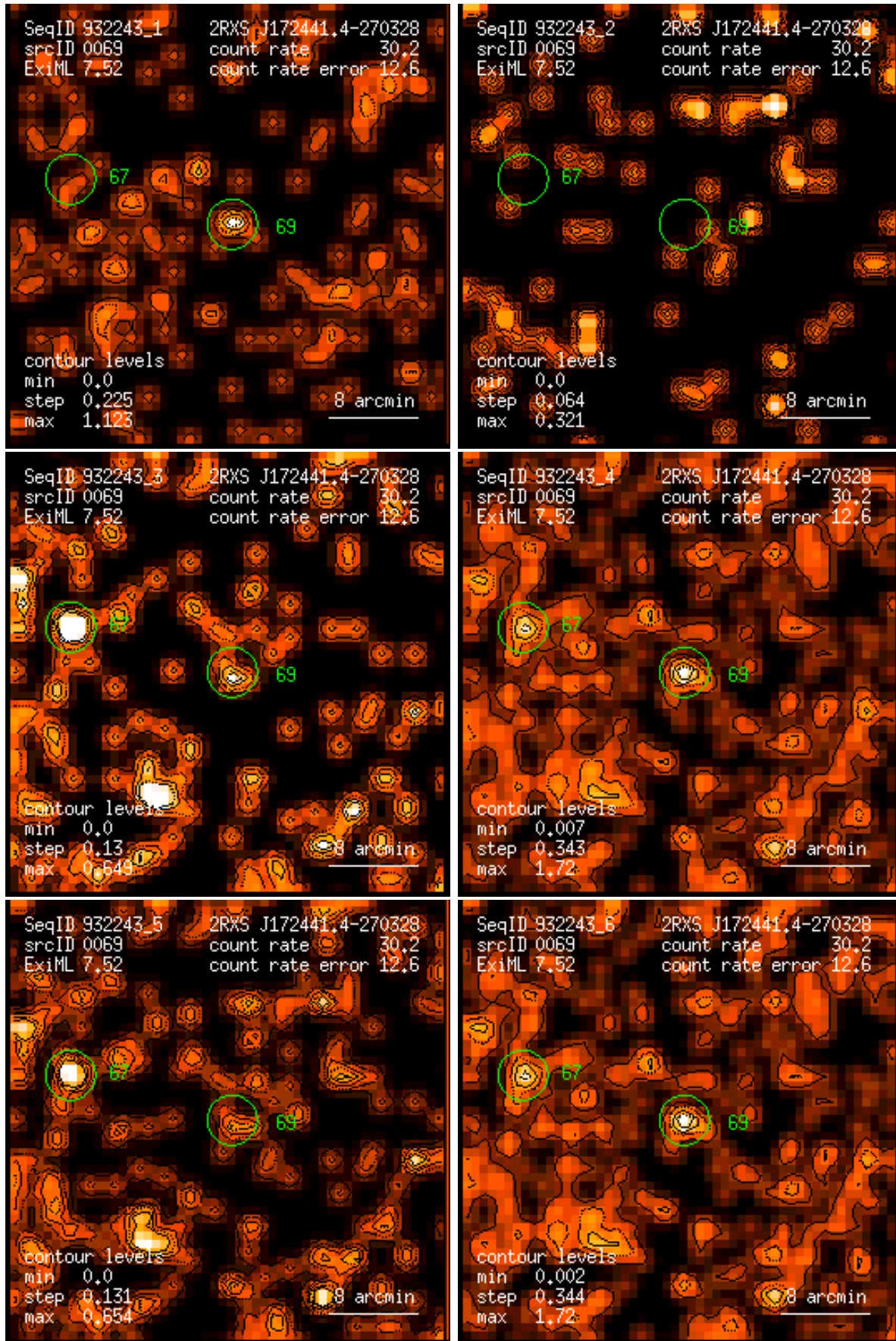
Figure 69: RASS 932243: detection 0069: band rate images, Gaussian filter: (1) PSPC channels 11 – 41, (2) 52 – 90, (3) 91 – 201, (4) 11 – 235, (5) 52 – 201, (6) 11 – 201. Broad band rates in counts/ks. Band rate contour levels in counts/ks/arcmin 2 .
