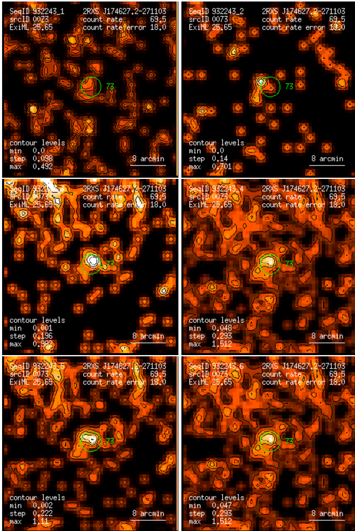
Figure 73: RASS 932243: detection 0073: band rate images, Gaussian filter: (1) PSPC channels 11 – 41, (2) 52 – 90, (3) 91 – 201, (4) 11 – 235, (5) 52 – 201, (6) 11 – 201. Broad band rates in counts/ks. Band rate contour levels in counts/ks/arcmin 2 .
