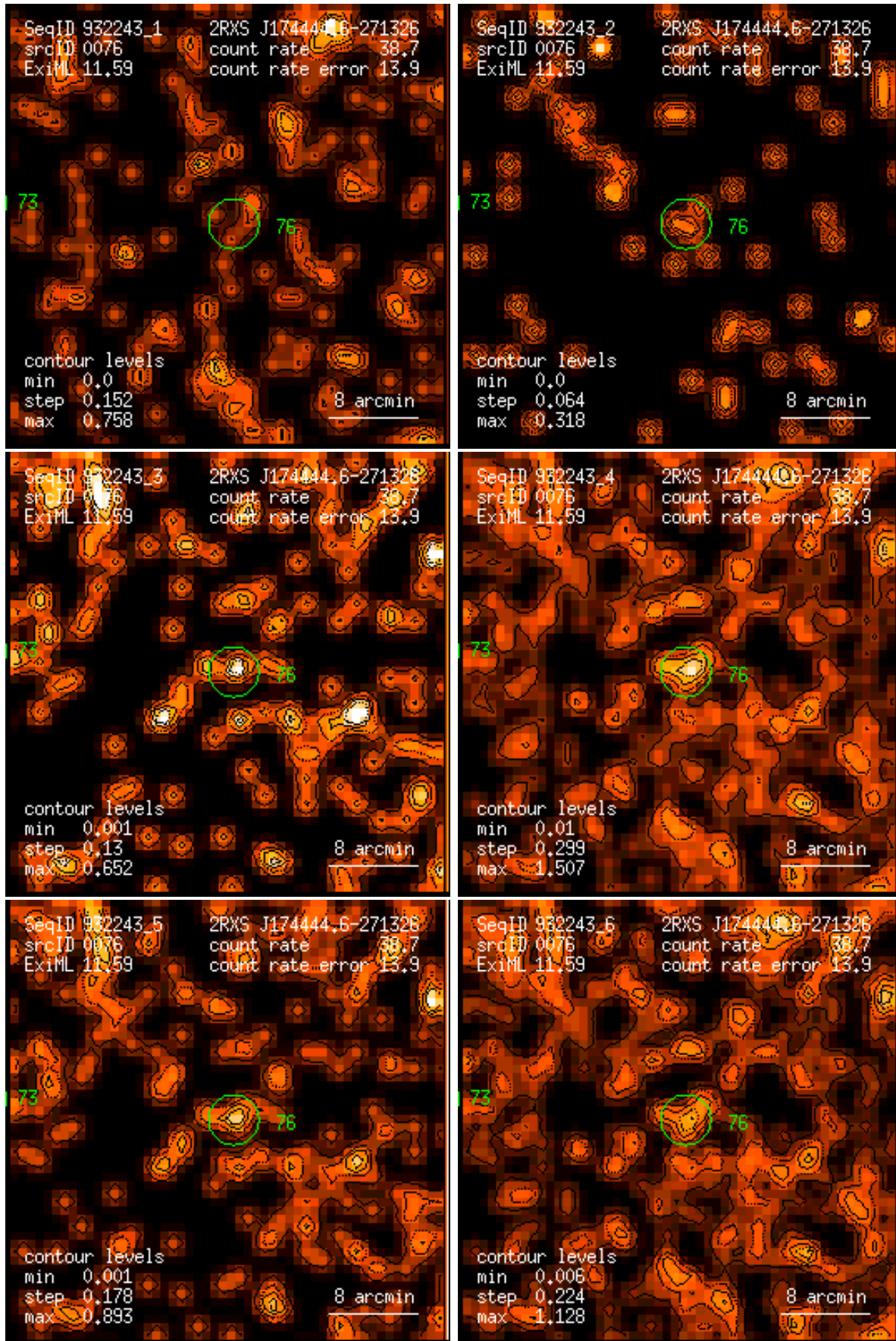
Figure 76: RASS 932243: detection 0076: band rate images, Gaussian filter: (1) PSPC channels 11 – 41, (2) 52 – 90, (3) 91 – 201, (4) 11 – 235, (5) 52 – 201, (6) 11 – 201. Broad band rates in counts/ks. Band rate contour levels in counts/ks/arcmin 2 .
