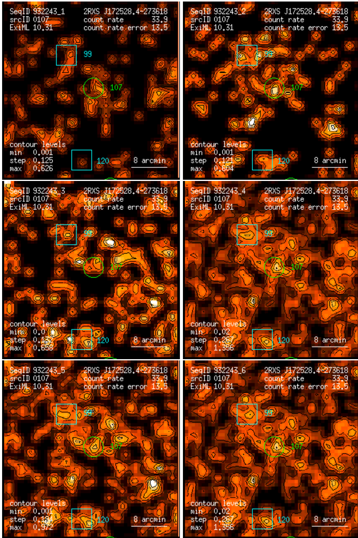
Figure 107: RASS 932243: detection 0107: band rate images, Gaussian filter: (1) PSPC channels 11 – 41, (2) 52 – 90, (3) 91 – 201, (4) 11 – 235, (5) 52 – 201, (6) 11 – 201. Broad band rates in counts/ks. Band rate contour levels in counts/ks/arcmin 2 .
