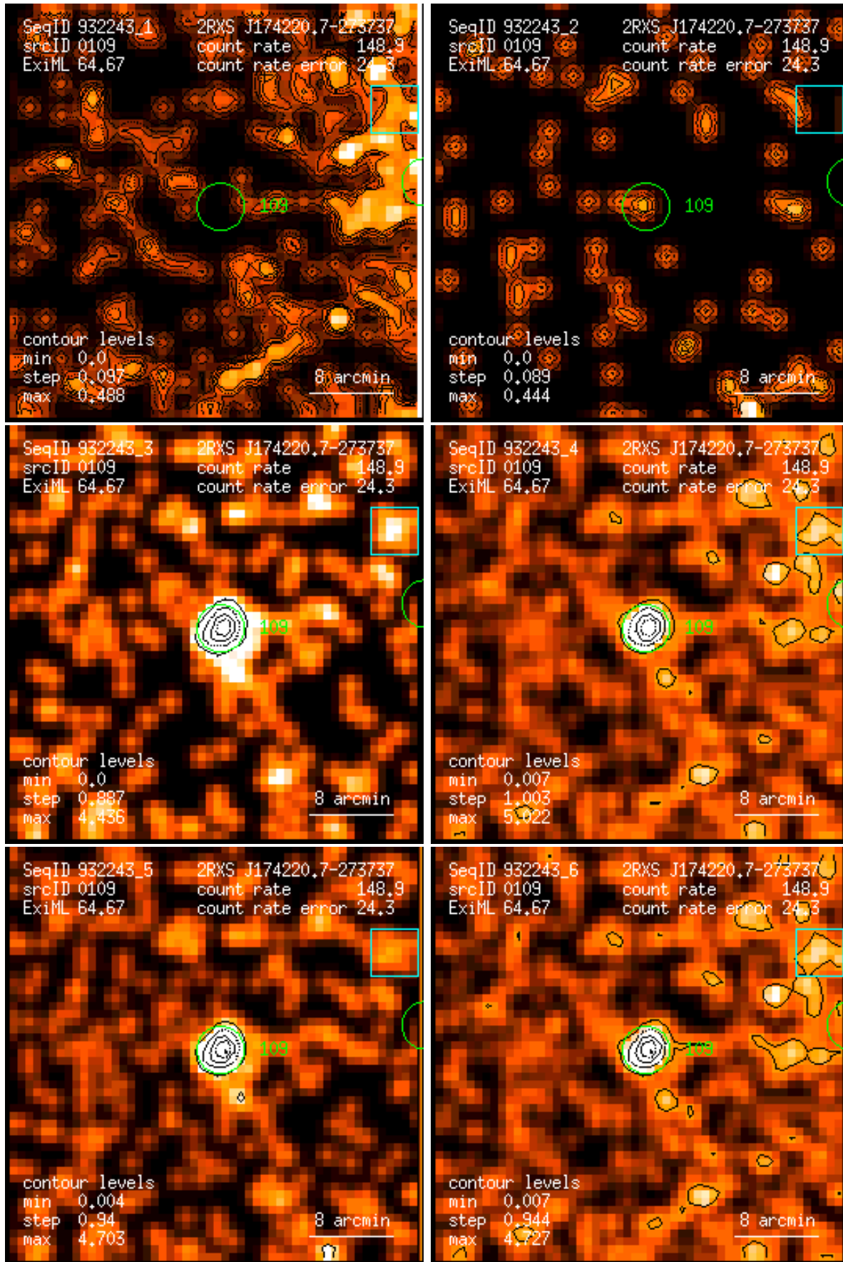
Figure 109: RASS 932243: detection 0109: band rate images, Gaussian filter: (1) PSPC channels 11 – 41, (2) 52 – 90, (3) 91 – 201, (4) 11 – 235, (5) 52 – 201, (6) 11 – 201. Broad band rates in counts/ks. Band rate contour levels in counts/ks/arcmin 2 .
