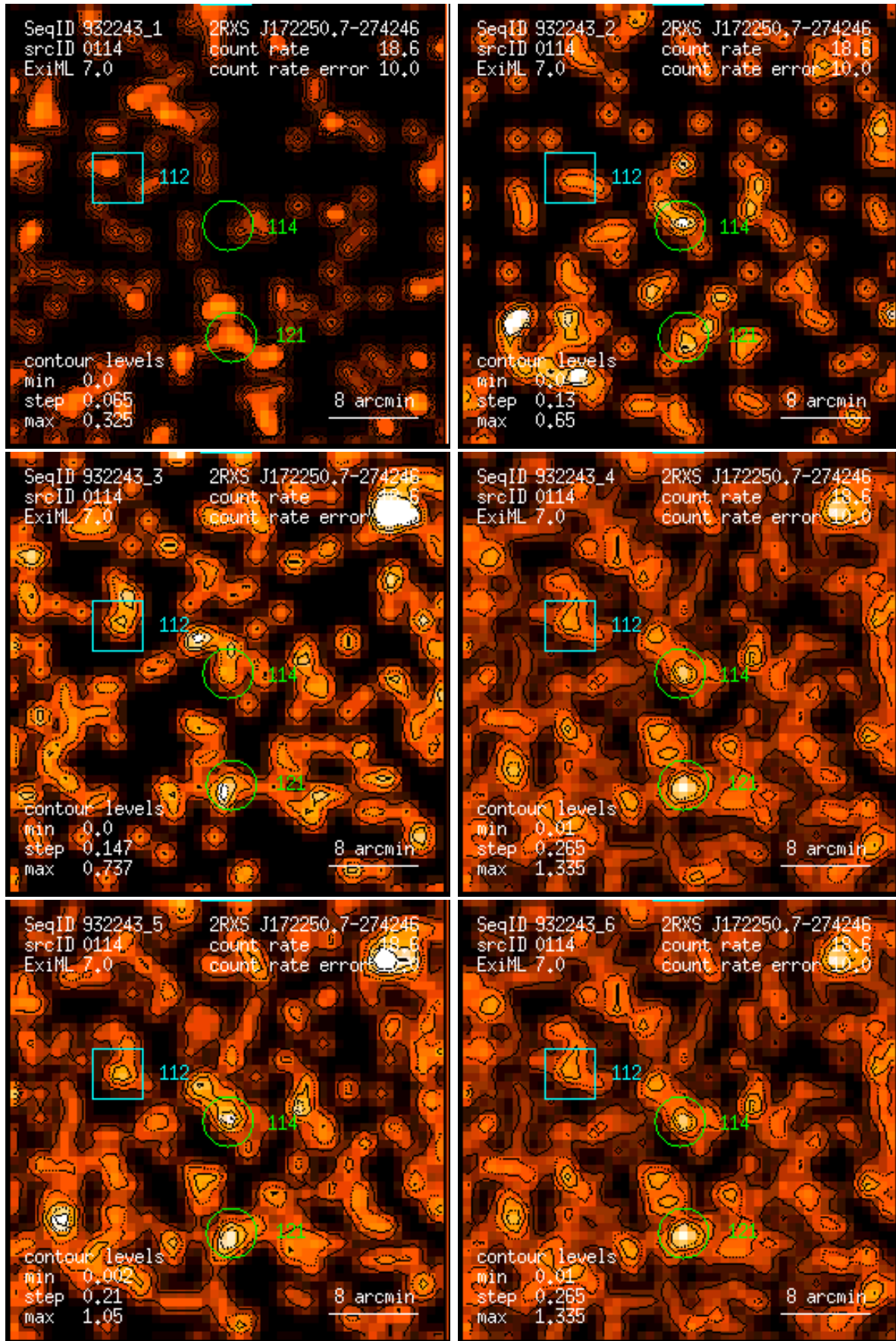
Figure 114: RASS 932243: detection 0114: band rate images, Gaussian filter: (1) PSPC channels 11 – 41, (2) 52 – 90, (3) 91 – 201, (4) 11 – 235, (5) 52 – 201, (6) 11 – 201. Broad band rates in counts/ks. Band rate contour levels in counts/ks/arcmin 2 .
