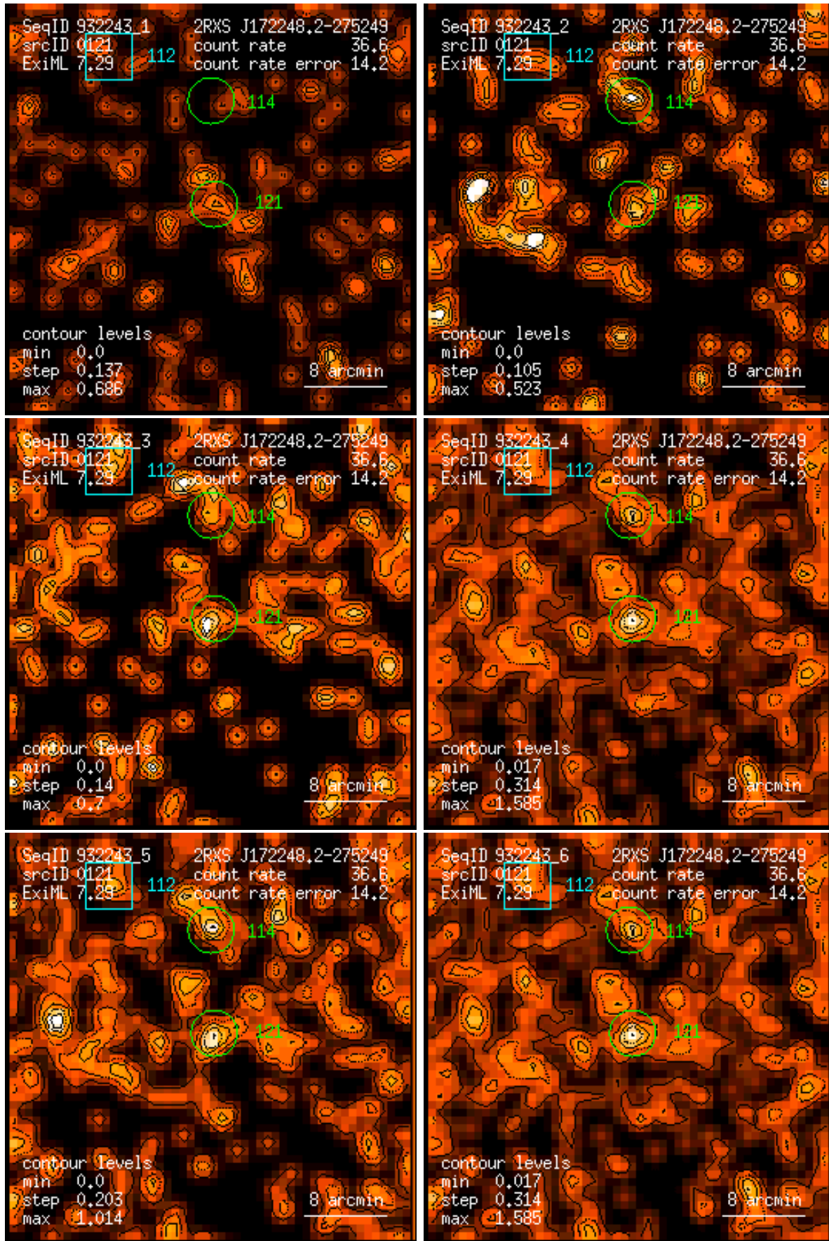
Figure 121: RASS 932243: detection 0121: band rate images, Gaussian filter: (1) PSPC channels 11 – 41, (2) 52 – 90, (3) 91 – 201, (4) 11 – 235, (5) 52 – 201, (6) 11 – 201. Broad band rates in counts/ks. Band rate contour levels in counts/ks/arcmin 2 .
