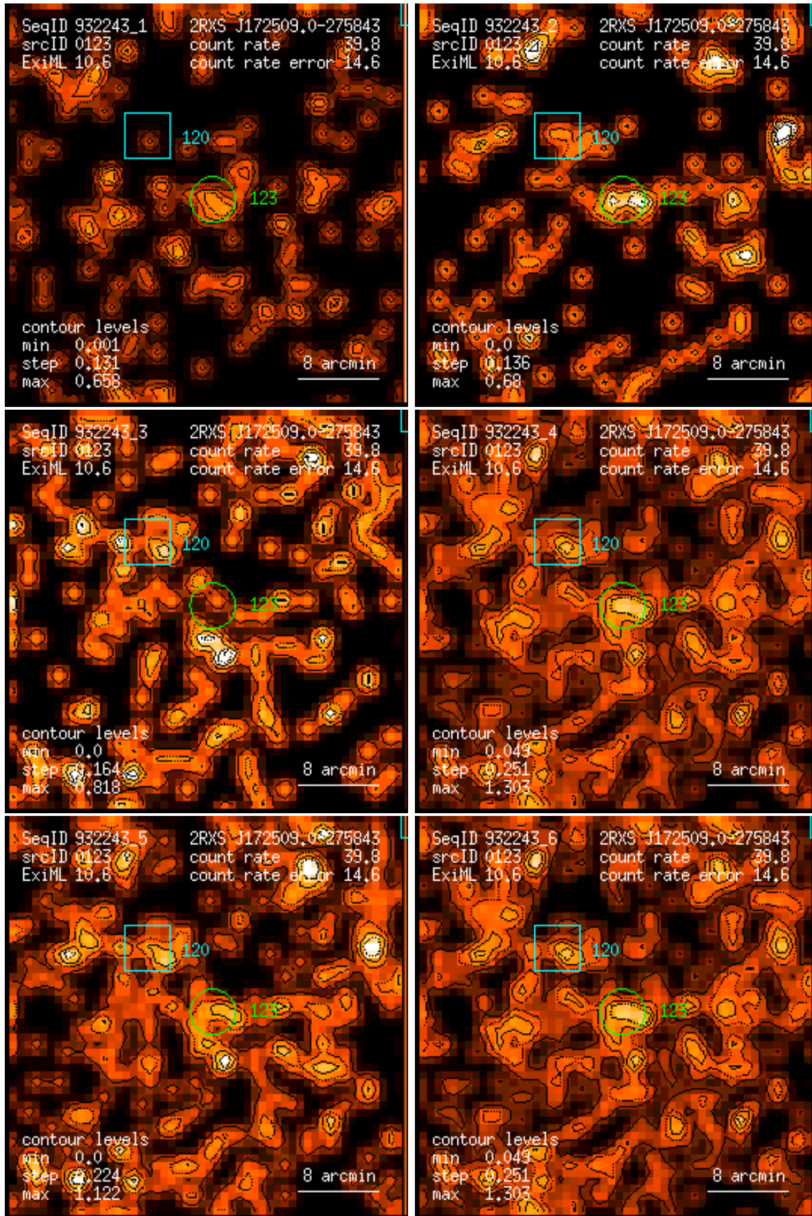
Figure 123: RASS 932243: detection 0123: band rate images, Gaussian filter: (1) PSPC channels 11 – 41, (2) 52 – 90, (3) 91 – 201, (4) 11 – 235, (5) 52 – 201, (6) 11 – 201. Broad band rates in counts/ks. Band rate contour levels in counts/ks/arcmin 2 .
