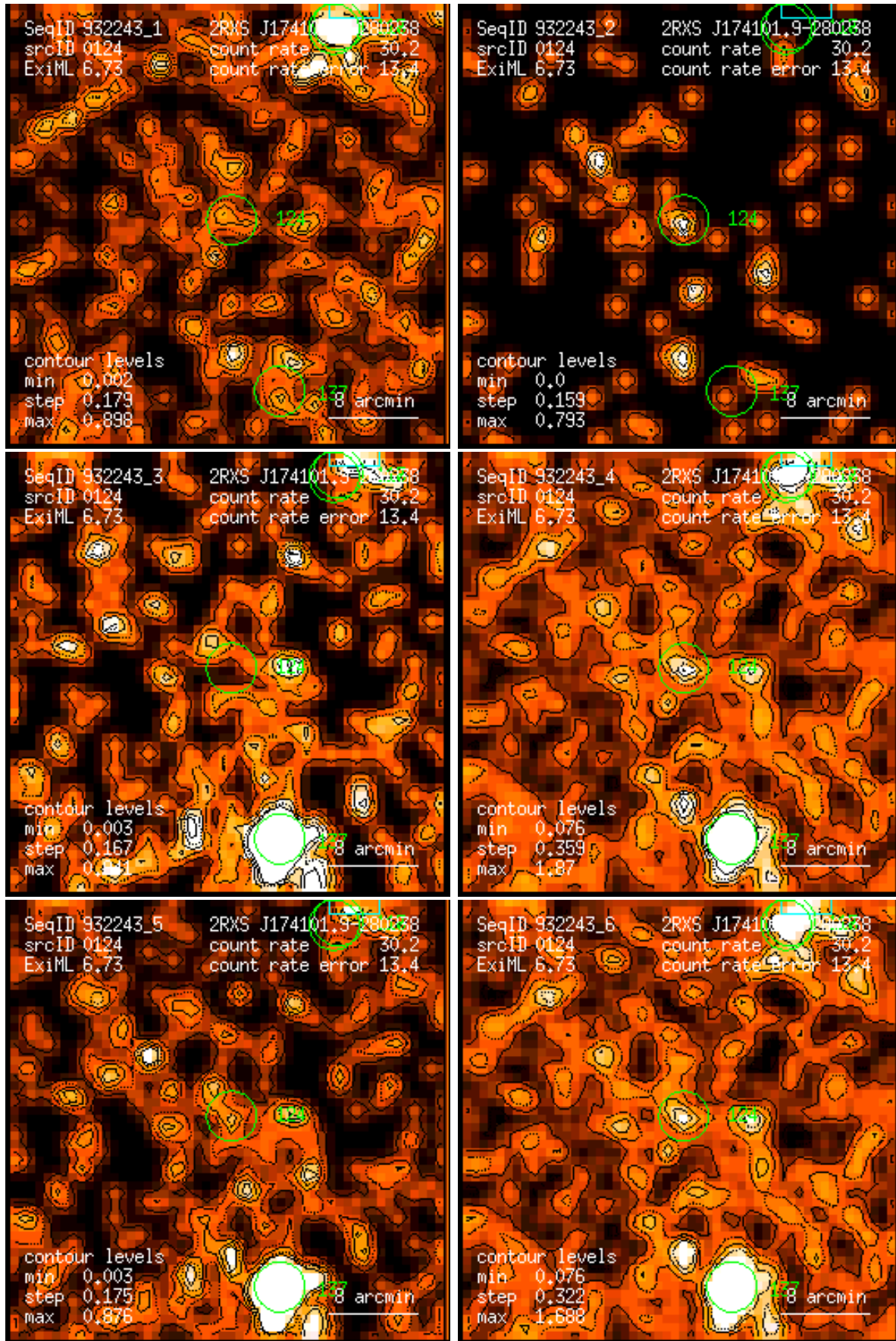
Figure 124: RASS 932243: detection 0124: band rate images, Gaussian filter: (1) PSPC channels 11 – 41, (2) 52 – 90, (3) 91 – 201, (4) 11 – 235, (5) 52 – 201, (6) 11 – 201. Broad band rates in counts/ks. Band rate contour levels in counts/ks/arcmin 2 .
