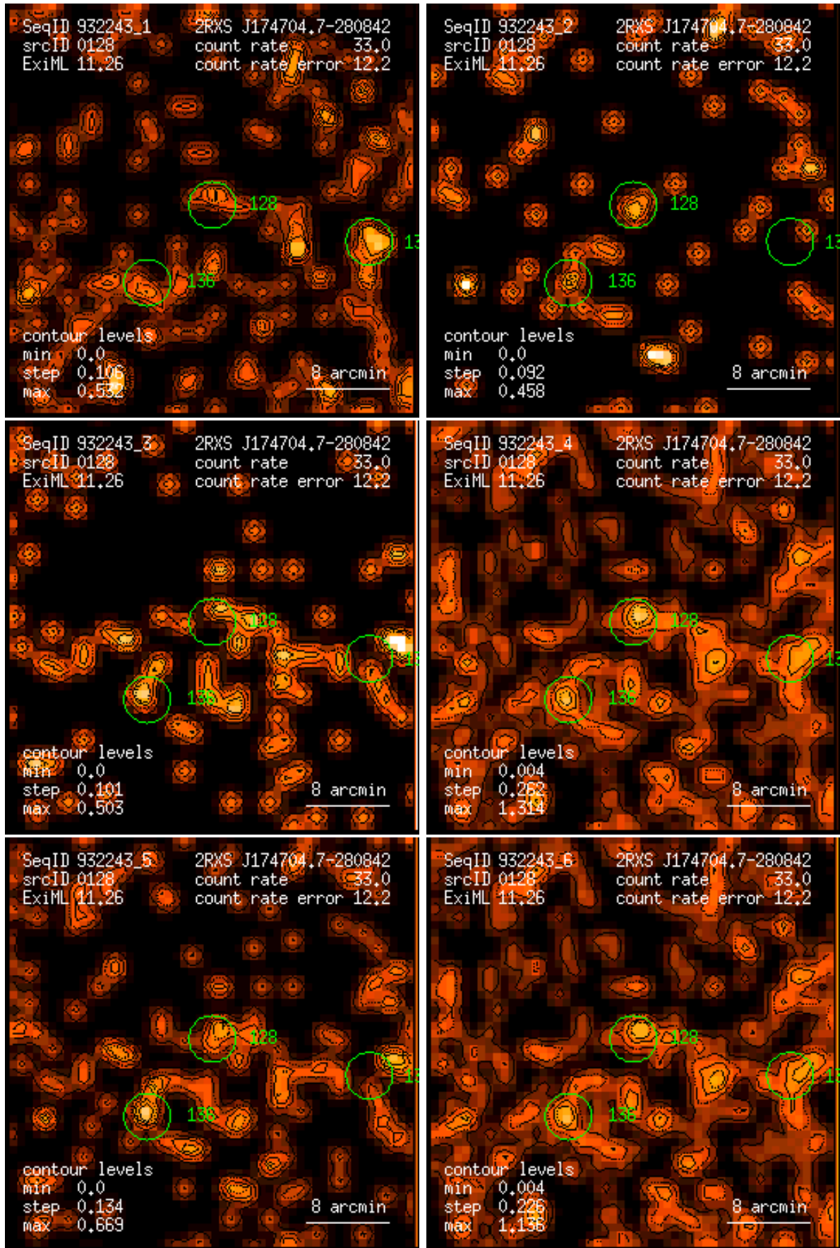
Figure 128: RASS 932243: detection 0128: band rate images, Gaussian filter: (1) PSPC channels 11 – 41, (2) 52 – 90, (3) 91 – 201, (4) 11 – 235, (5) 52 – 201, (6) 11 – 201. Broad band rates in counts/ks. Band rate contour levels in counts/ks/arcmin 2 .
