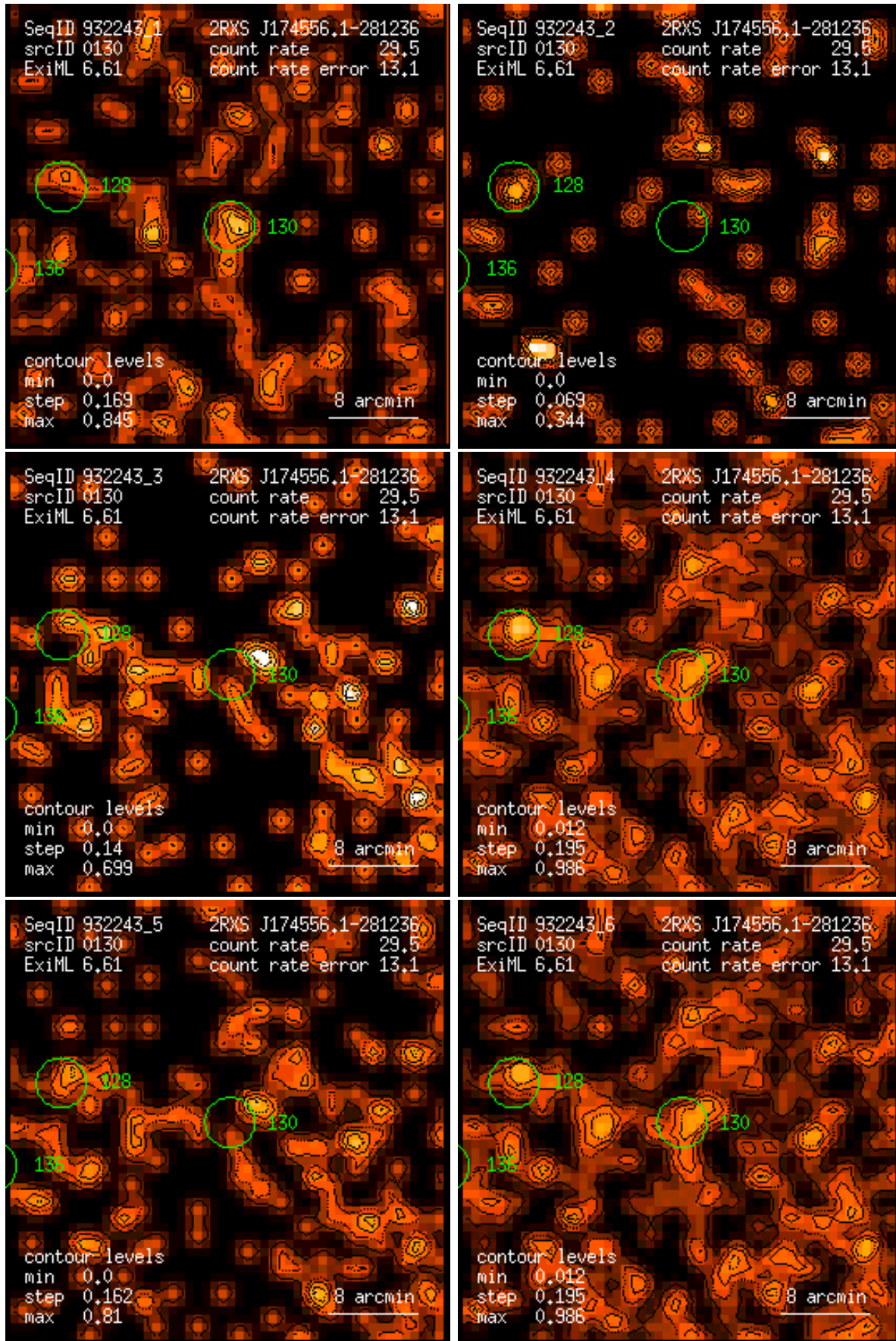
Figure 130: RASS 932243: detection 0130: band rate images, Gaussian filter: (1) PSPC channels 11 – 41, (2) 52 – 90, (3) 91 – 201, (4) 11 – 235, (5) 52 – 201, (6) 11 – 201. Broad band rates in counts/ks. Band rate contour levels in counts/ks/arcmin 2 .
