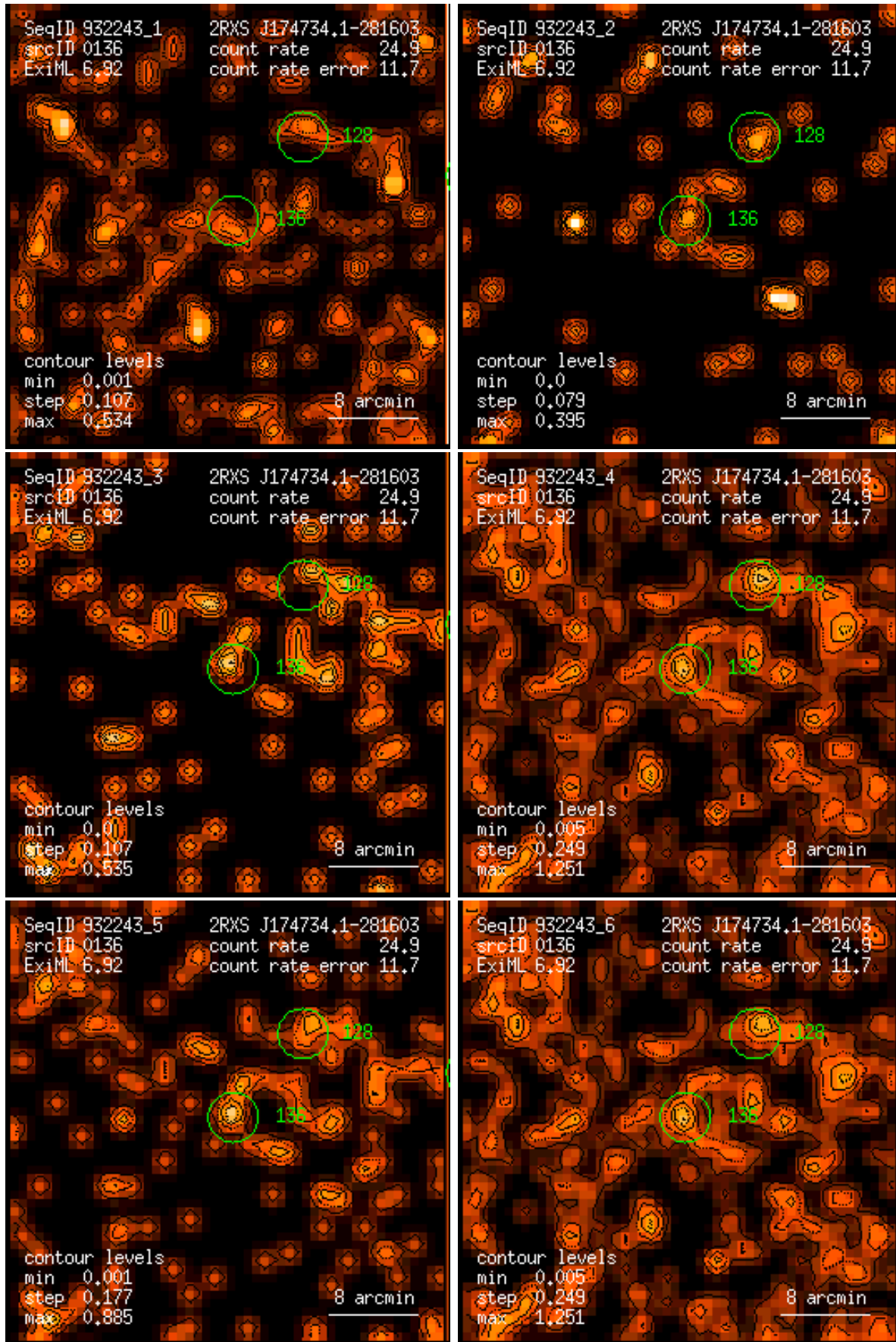
Figure 136: RASS 932243: detection 0136: band rate images, Gaussian filter: (1) PSPC channels 11 – 41, (2) 52 – 90, (3) 91 – 201, (4) 11 – 235, (5) 52 – 201, (6) 11 – 201. Broad band rates in counts/ks. Band rate contour levels in counts/ks/arcmin 2 .
