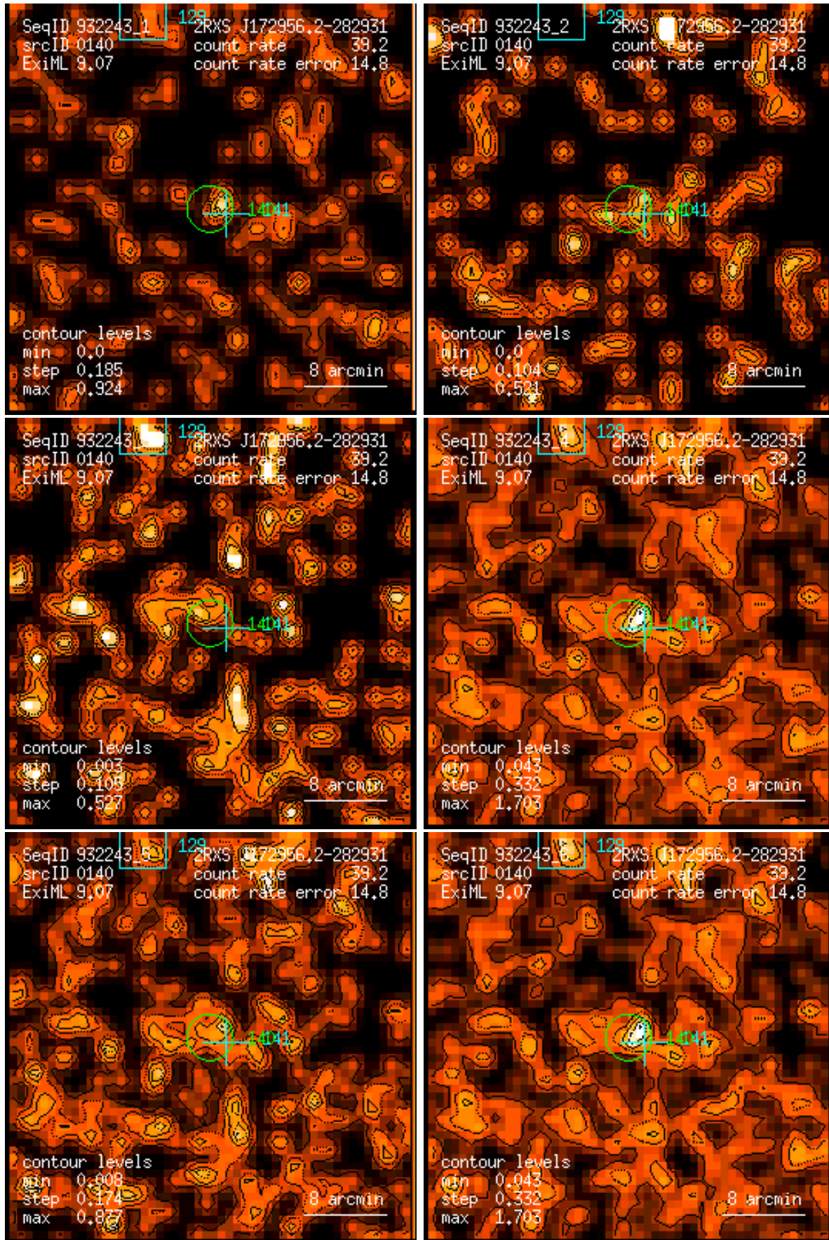
Figure 140: RASS 932243: detection 0140: band rate images, Gaussian filter: (1) PSPC channels 11 – 41, (2) 52 – 90, (3) 91 – 201, (4) 11 – 235, (5) 52 – 201, (6) 11 – 201. Broad band rates in counts/ks. Band rate contour levels in counts/ks/arcmin 2 .
