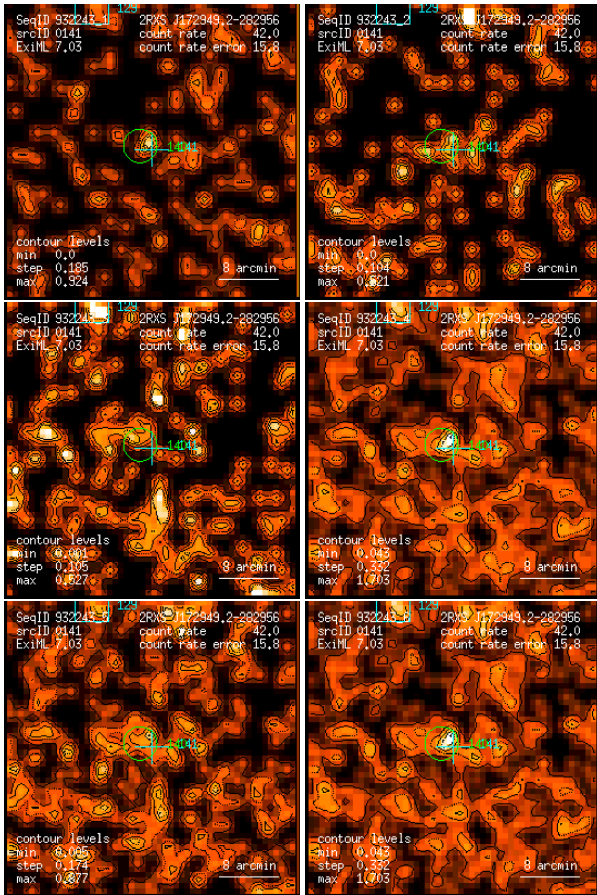
Figure 141: RASS 932243: detection 0141: band rate images, Gaussian filter: (1) PSPC channels 11 – 41, (2) 52 – 90, (3) 91 – 201, (4) 11 – 235, (5) 52 – 201, (6) 11 – 201. Broad band rates in counts/ks. Band rate contour levels in counts/ks/arcmin 2 .
