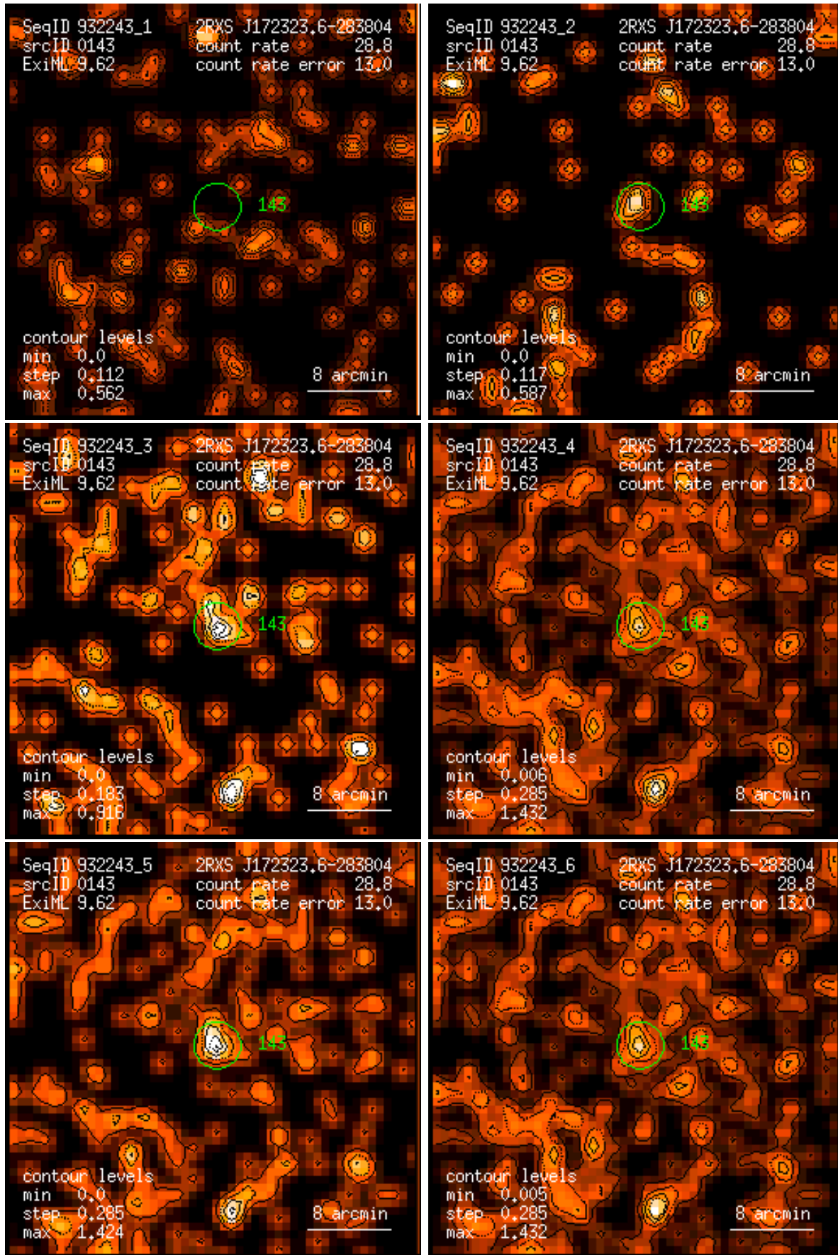
Figure 143: RASS 932243: detection 0143: band rate images, Gaussian filter: (1) PSPC channels 11 – 41, (2) 52 – 90, (3) 91 – 201, (4) 11 – 235, (5) 52 – 201, (6) 11 – 201. Broad band rates in counts/ks. Band rate contour levels in counts/ks/arcmin 2 .
