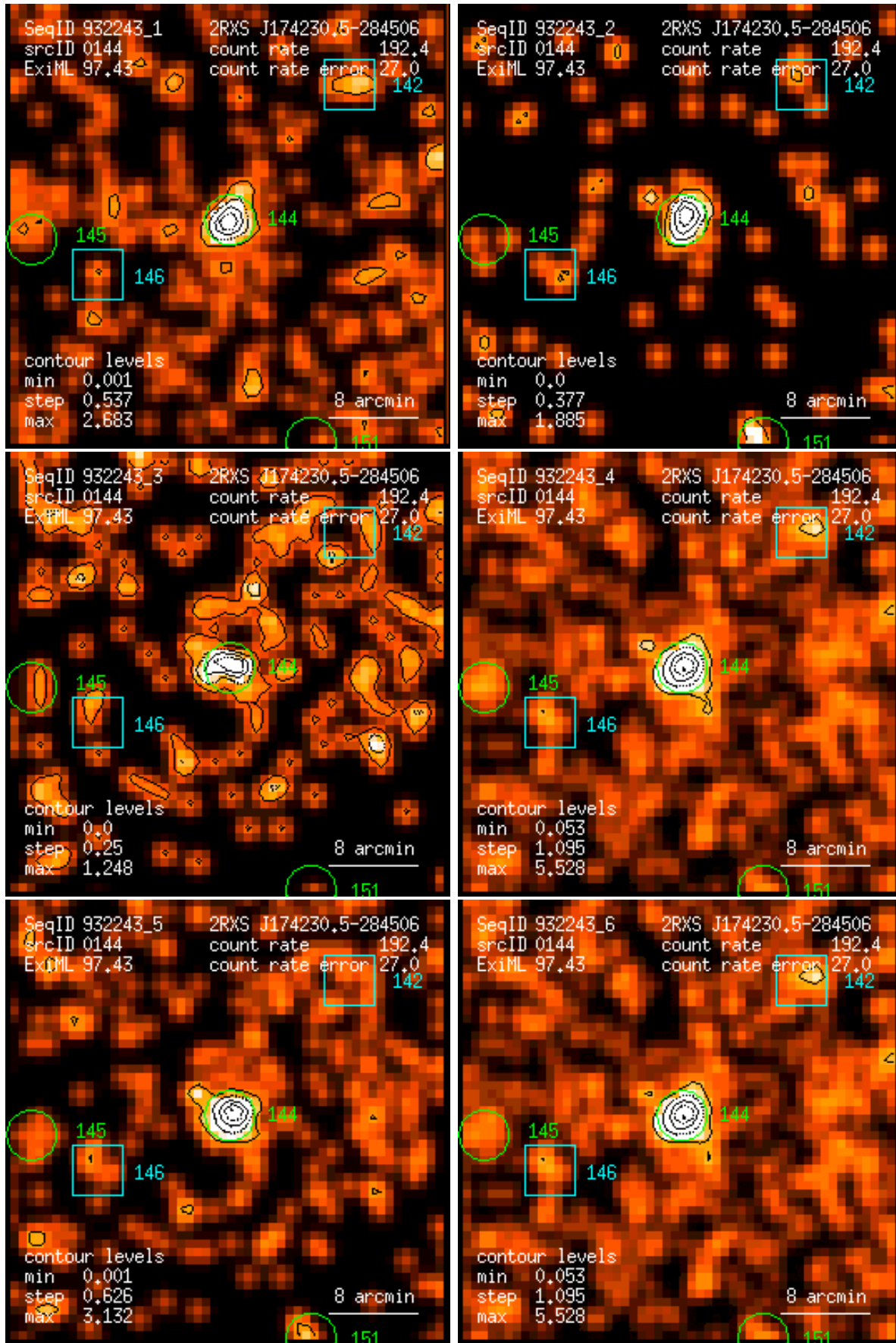
Figure 144: RASS 932243: detection 0144: band rate images, Gaussian filter: (1) PSPC channels 11 – 41, (2) 52 – 90, (3) 91 – 201, (4) 11 – 235, (5) 52 – 201, (6) 11 – 201. Broad band rates in counts/ks. Band rate contour levels in counts/ks/arcmin 2 .
