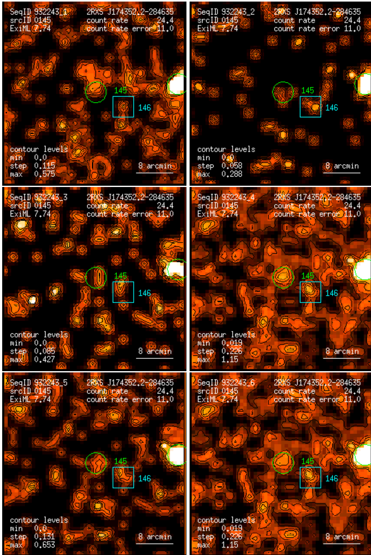
Figure 145: RASS 932243: detection 0145: band rate images, Gaussian filter: (1) PSPC channels 11 – 41, (2) 52 – 90, (3) 91 – 201, (4) 11 – 235, (5) 52 – 201, (6) 11 – 201. Broad band rates in counts/ks. Band rate contour levels in counts/ks/arcmin 2 .
