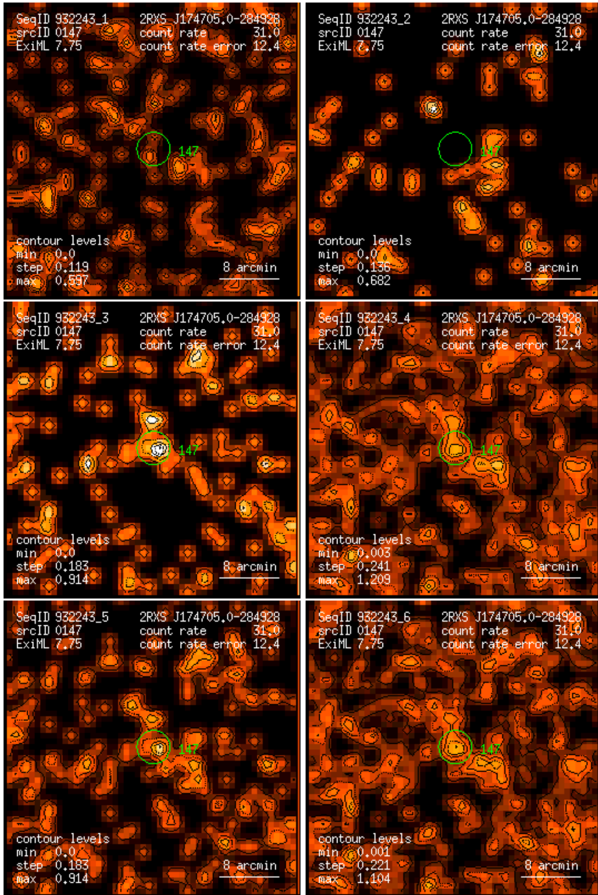
Figure 147: RASS 932243: detection 0147: band rate images, Gaussian filter: (1) PSPC channels 11 – 41, (2) 52 – 90, (3) 91 – 201, (4) 11 – 235, (5) 52 – 201, (6) 11 – 201. Broad band rates in counts/ks. Band rate contour levels in counts/ks/arcmin 2 .
