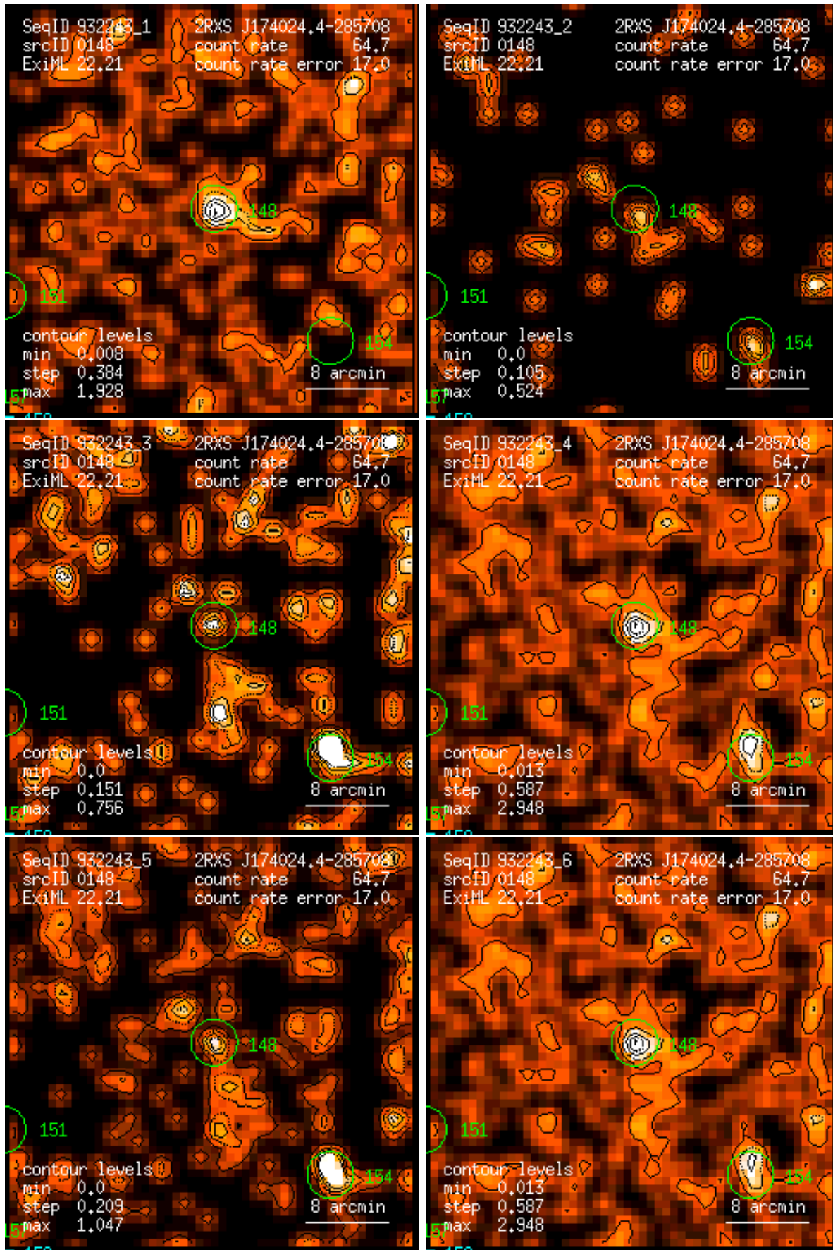
Figure 148: RASS 932243: detection 0148: band rate images, Gaussian filter: (1) PSPC channels 11 – 41, (2) 52 – 90, (3) 91 – 201, (4) 11 – 235, (5) 52 – 201, (6) 11 – 201. Broad band rates in counts/ks. Band rate contour levels in counts/ks/arcmin 2 .
