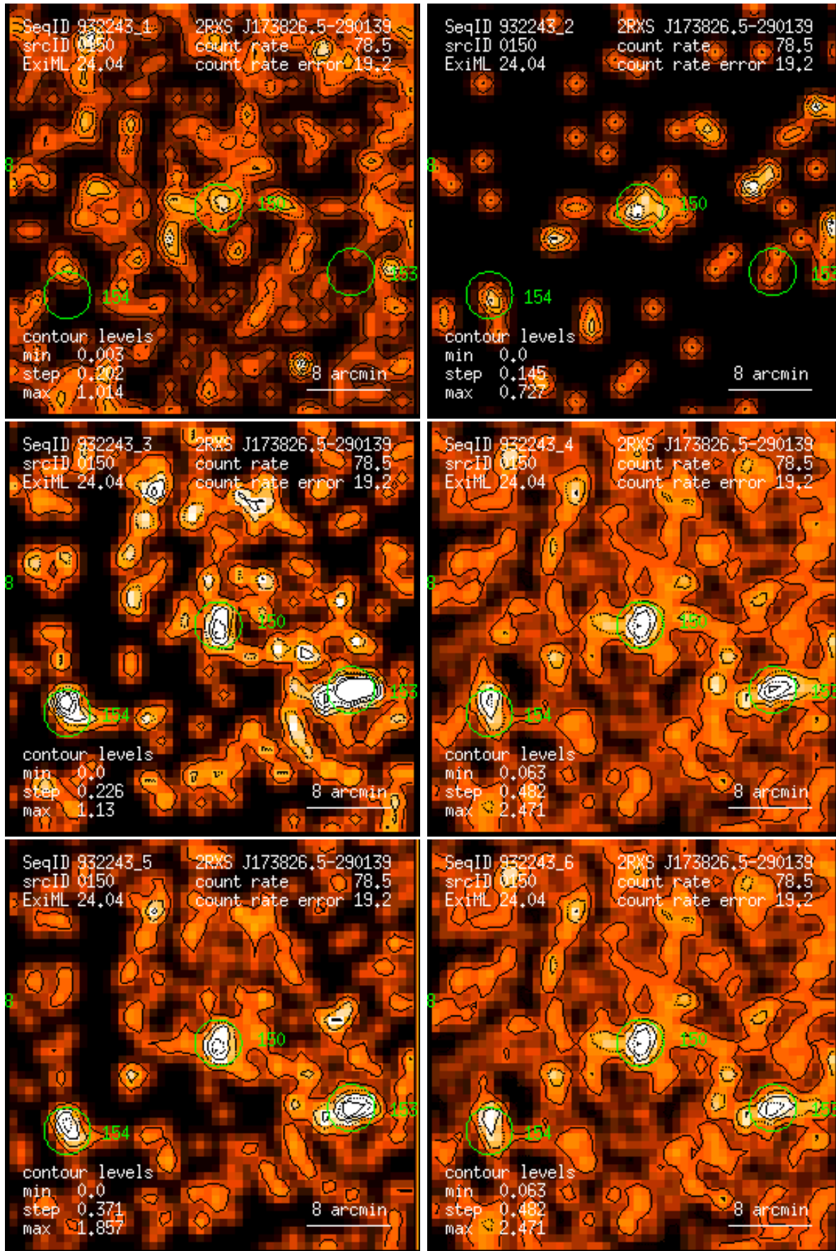
Figure 150: RASS 932243: detection 0150: band rate images, Gaussian filter: (1) PSPC channels 11 – 41, (2) 52 – 90, (3) 91 – 201, (4) 11 – 235, (5) 52 – 201, (6) 11 – 201. Broad band rates in counts/ks. Band rate contour levels in counts/ks/arcmin 2 .
