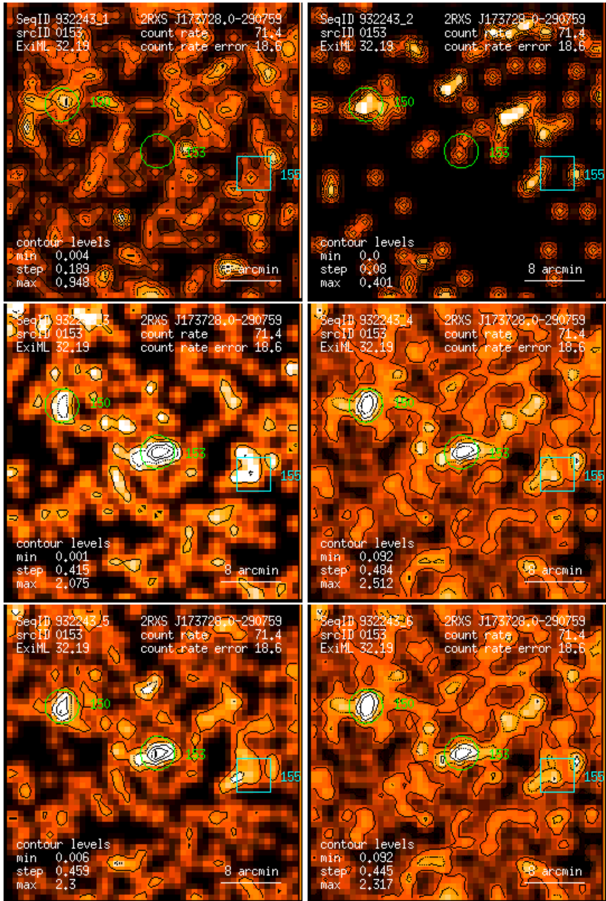
Figure 153: RASS 932243: detection 0153: band rate images, Gaussian filter: (1) PSPC channels 11 – 41, (2) 52 – 90, (3) 91 – 201, (4) 11 – 235, (5) 52 – 201, (6) 11 – 201. Broad band rates in counts/ks. Band rate contour levels in counts/ks/arcmin 2 .
