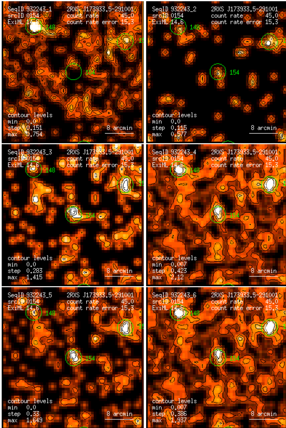
Figure 154: RASS 932243: detection 0154: band rate images, Gaussian filter: (1) PSPC channels 11 – 41, (2) 52 – 90, (3) 91 – 201, (4) 11 – 235, (5) 52 – 201, (6) 11 – 201. Broad band rates in counts/ks. Band rate contour levels in counts/ks/arcmin 2 .
