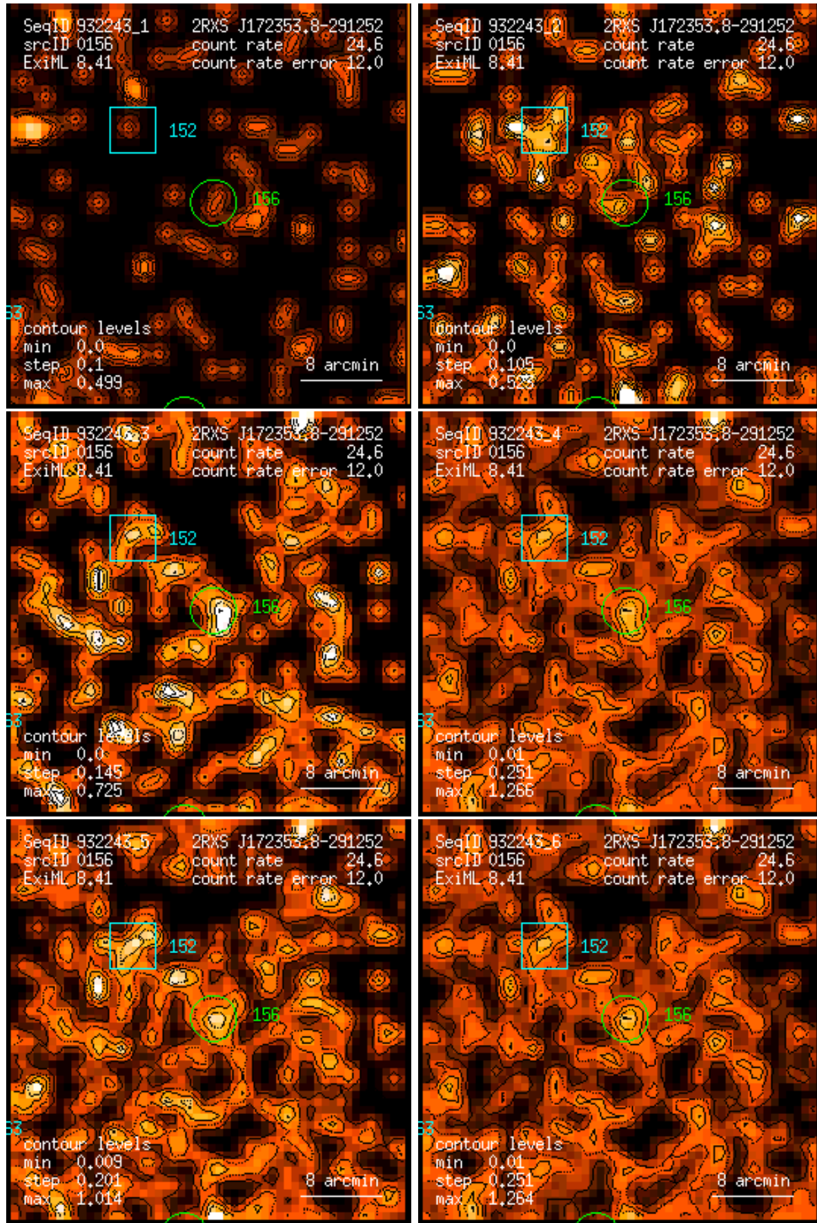
Figure 156: RASS 932243: detection 0156: band rate images, Gaussian filter: (1) PSPC channels 11 – 41, (2) 52 – 90, (3) 91 – 201, (4) 11 – 235, (5) 52 – 201, (6) 11 – 201. Broad band rates in counts/ks. Band rate contour levels in counts/ks/arcmin 2 .
